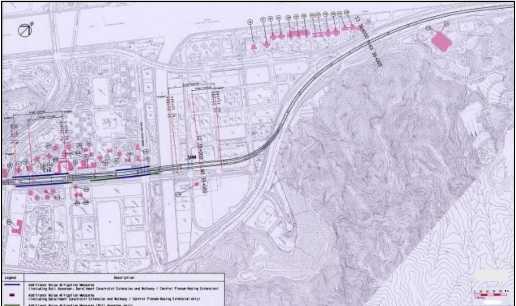
Figure 23 Locations of Additional Noise Mitigation Measures (Extracted from the Application VEP-157/2004)
