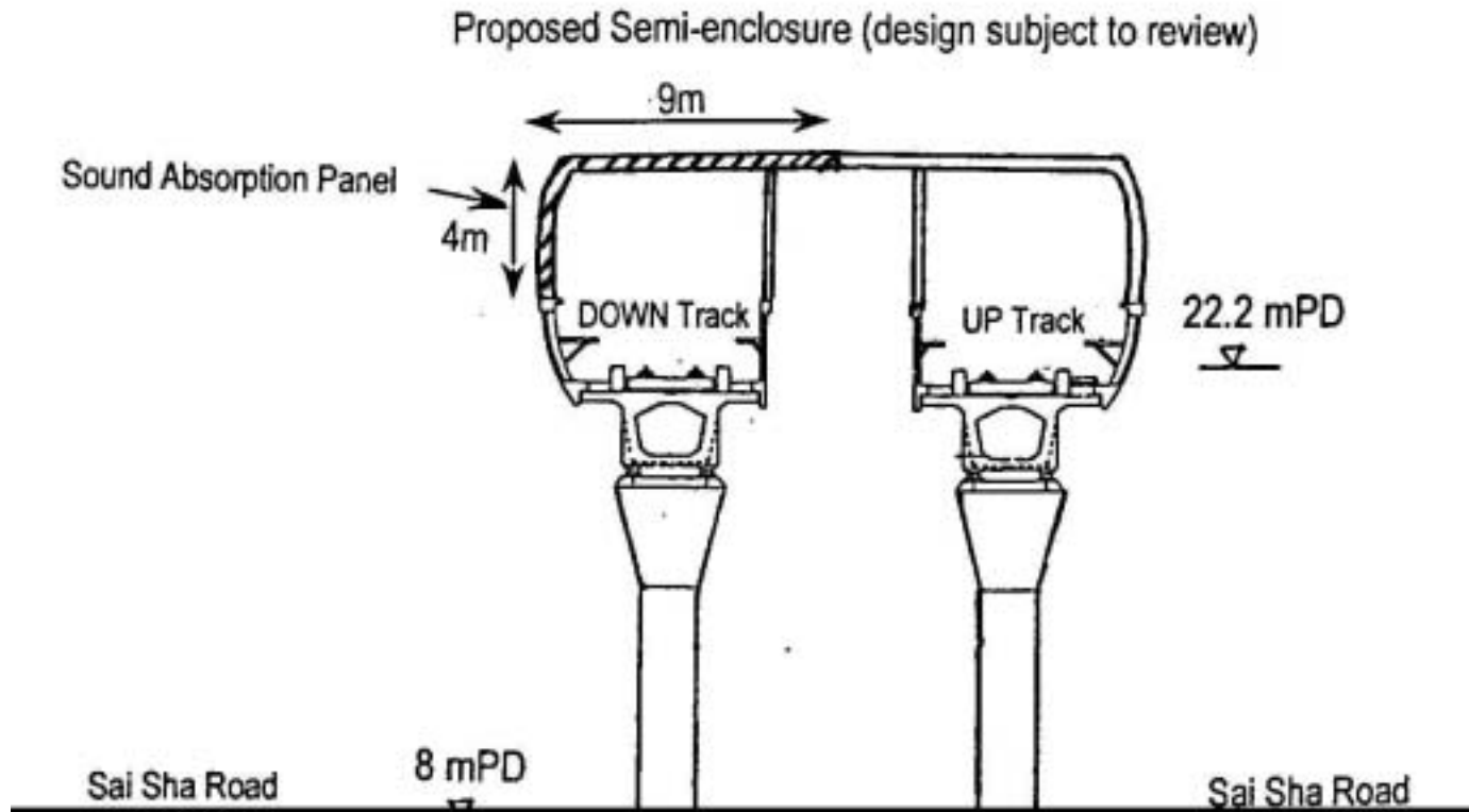
Figure 31 Semi-noise Enclosure Fronting Fok On Garden (Extracted from the Application VEP-157/2004)
