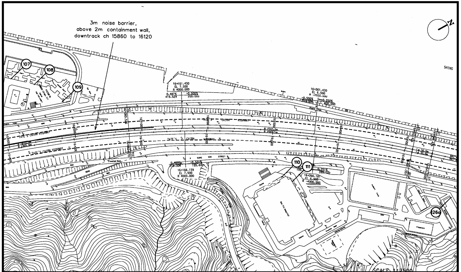
Figure 6 Noise Barriers and Enclosures (Extracted from Technical Annex F1 of the EIA Report)
