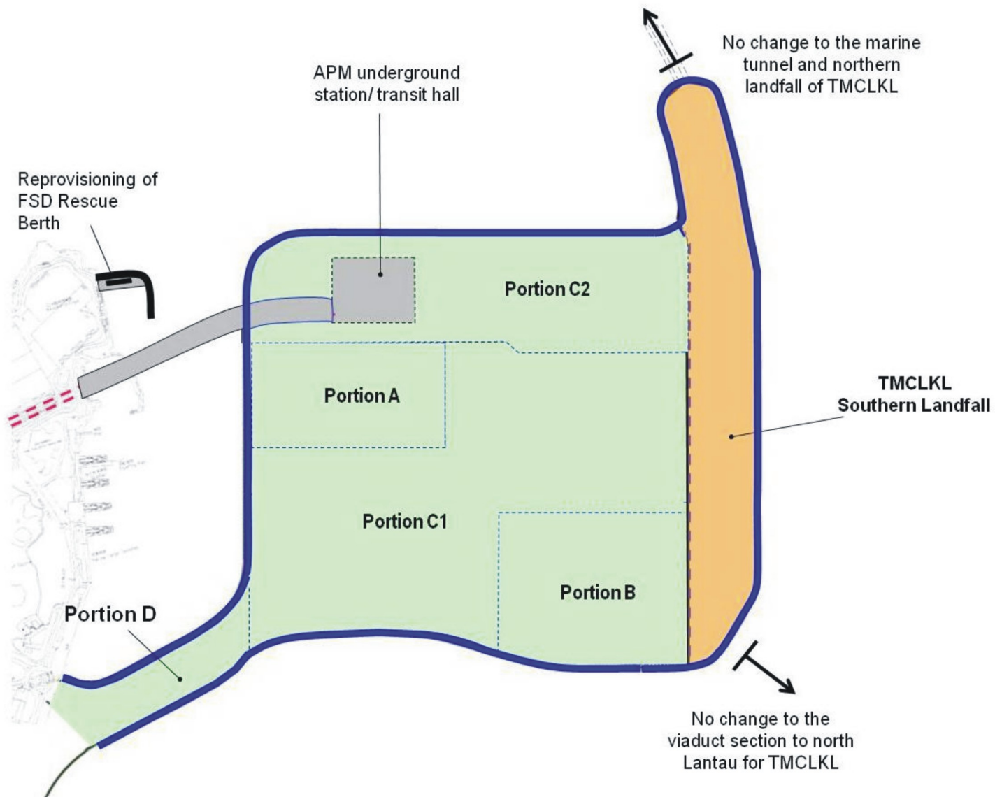
Figure 11 - Proposed Layout of HKBCF & TM-CLKL Southern Landfall Reclamation
