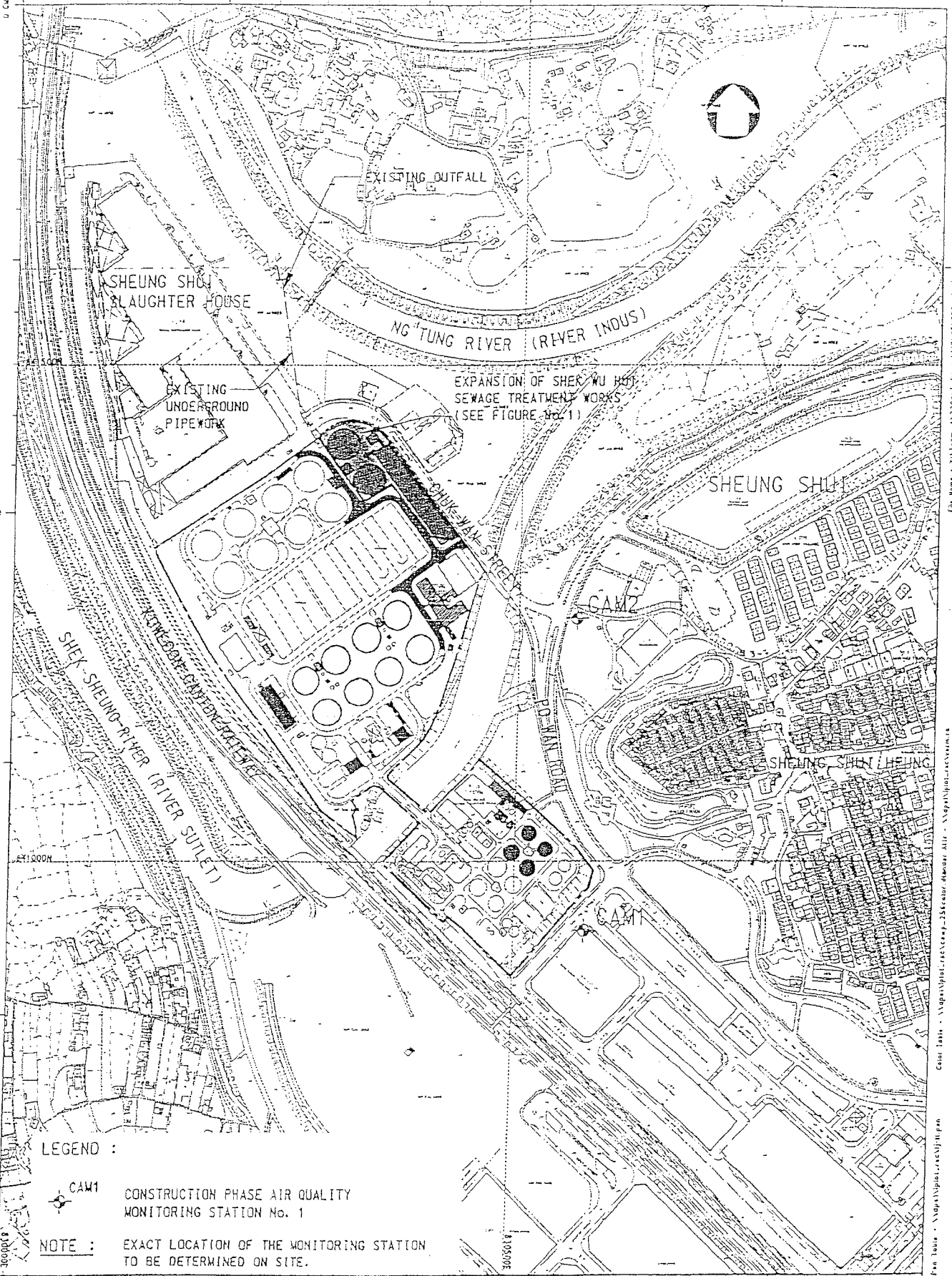
Figure Title EXPANSION OF SHEK WU HUI SEWAGE TREATMENT WORKS LOCATION PLAN OF PROPOSED AIR QUALITY MONITORING STATION FOR CONSTRUCTION PHASE
