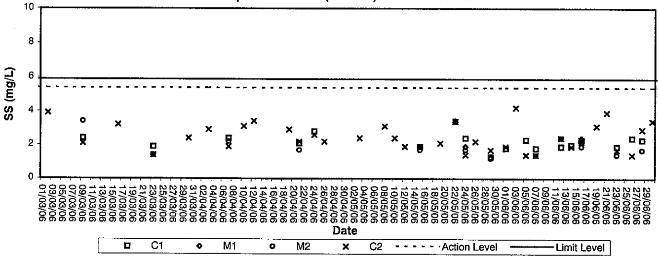
Suspended Solids (Surface) at mid-flood tide
