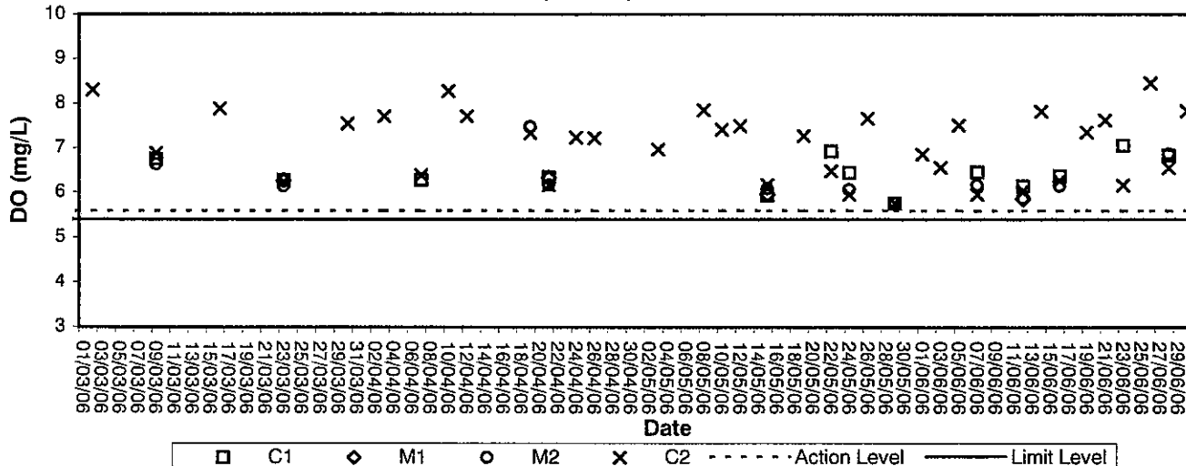
DO content (Bottom) at mid-ebb tide
