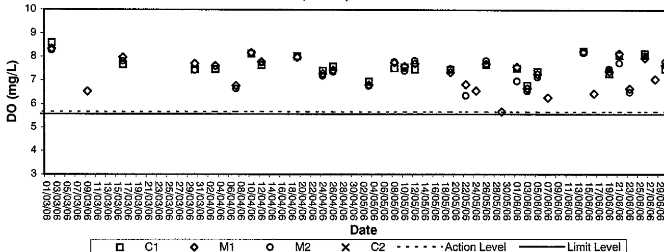
DO content (Middle) at mid-ebb tide
