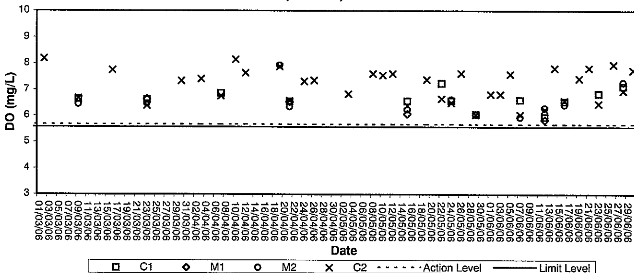
DO content (Surface) at mid-ebb tide
