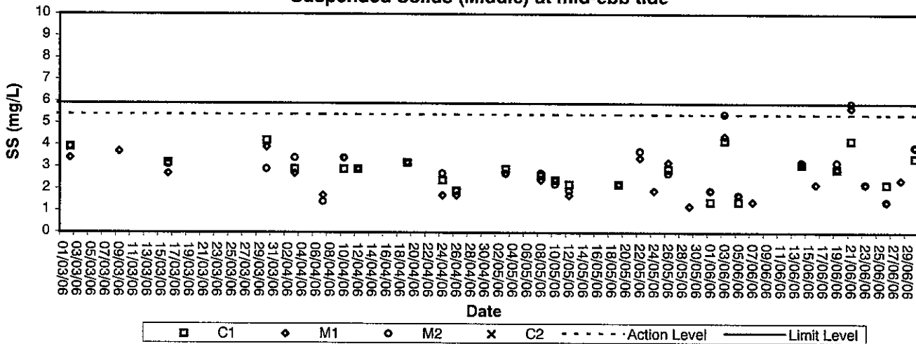
Suspended Solids (Middle) at mid-ebb tide
