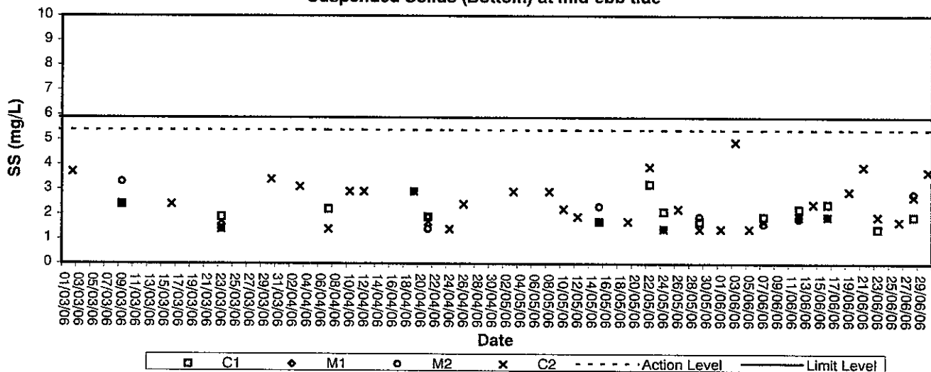
Suspended Solids (Bottom) at mid-ebb tide
