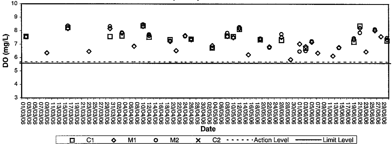
DO content (Middle) at mid-flood tide
