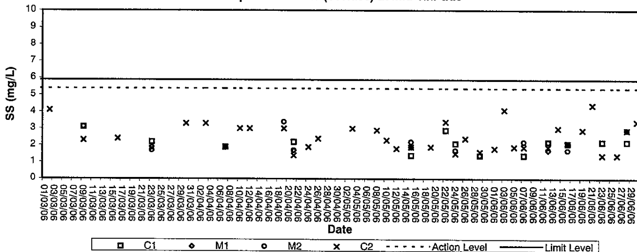
Suspended Solids (Surface) at mid-ebb tide
