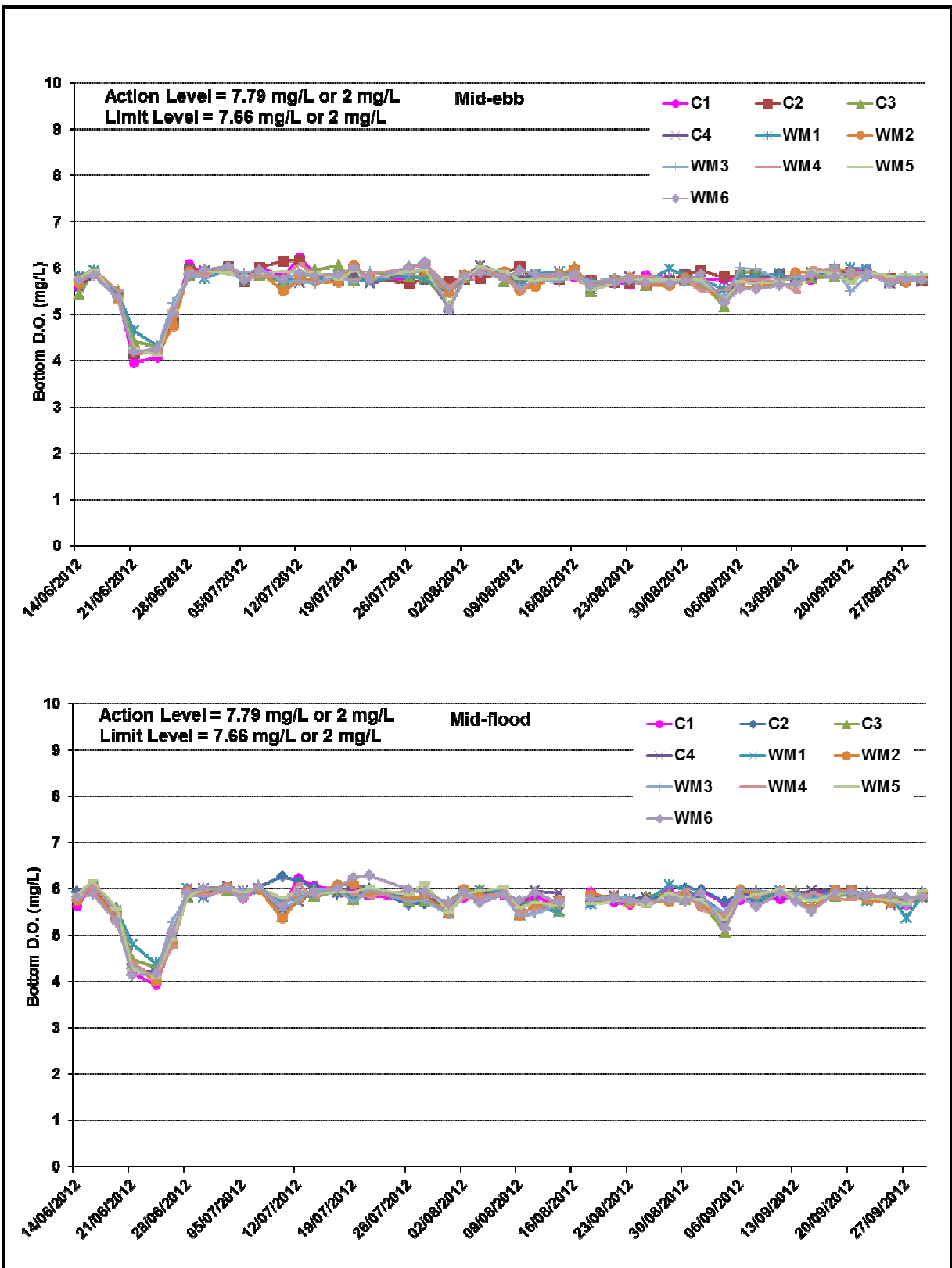
Figure B5 Impact Monitoring – Mean Level of Dissolved Oxygen (mg/L) in bottom waters between 14 June and 29 September 2012 at Monitoring Stations for Dredging Works.
