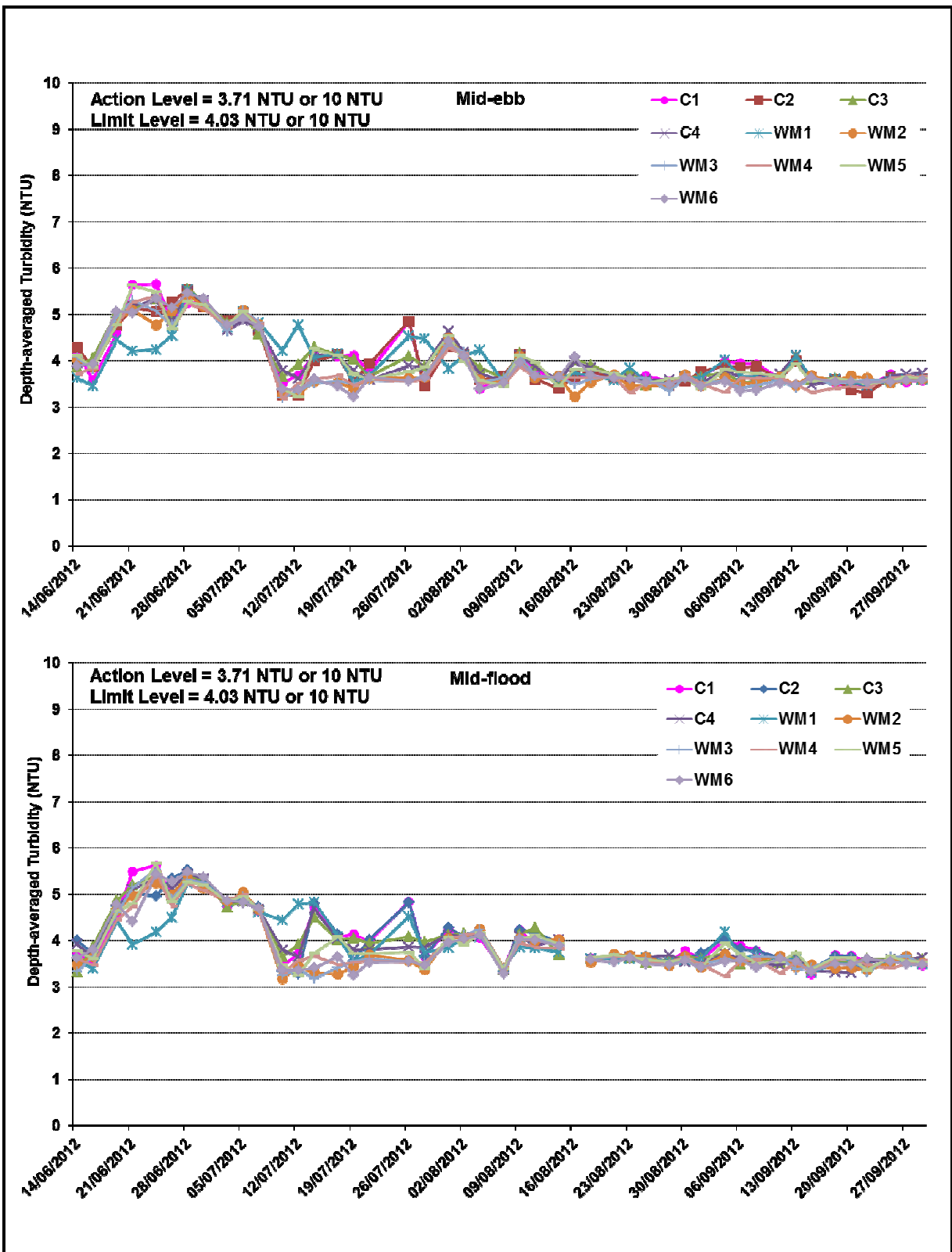
Figure B7 Impact Monitoring – Mean Depth-averaged Level of Turbidity (NTU) between 14 June and 29 September 2012 at Monitoring Stations for Dredging Works.
