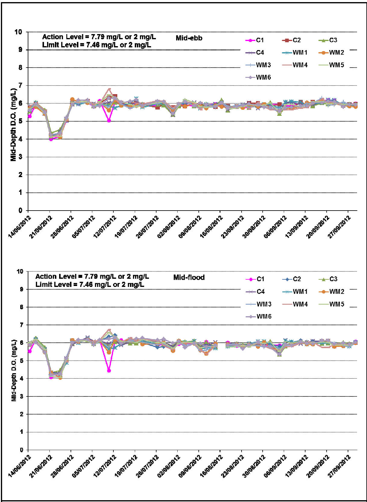
Figure B4 Impact Monitoring – Mean Level of Dissolved Oxygen (mg/L) in mid-depth waters between 14 June and 29 September 2012 at Monitoring Stations for Dredging Works.
