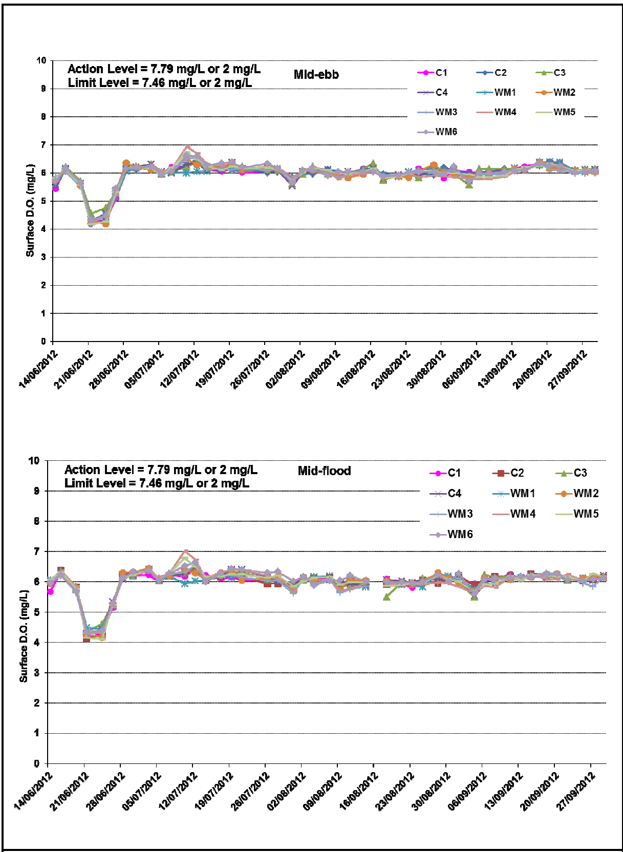
Figure B3 Impact Monitoring – Mean Level of Dissolved Oxygen (mg/L) in surface waters between 14 June and 29 September 2012 at Monitoring Stations for Dredging Works.
