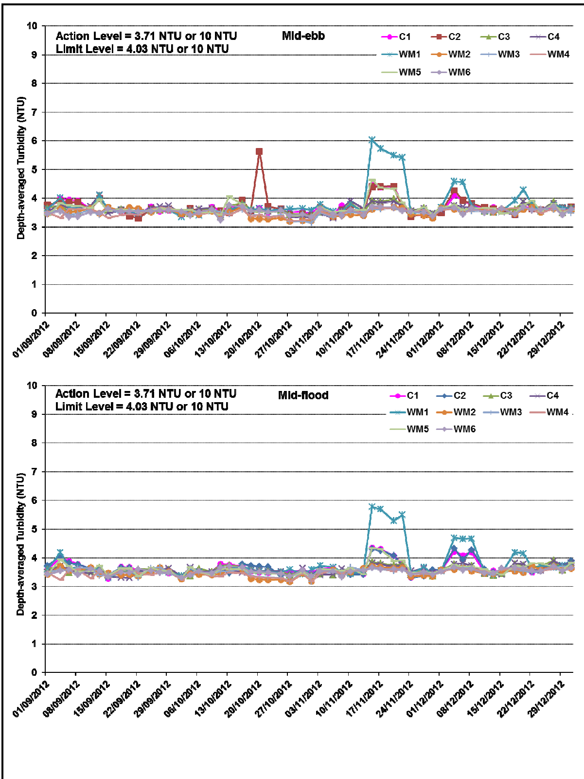
Figure B7 Impact Monitoring – Mean Depth-averaged Level of Turbidity (NTU) between 1 September and 31 December 2012 at Monitoring Stations for Dredging Works.
