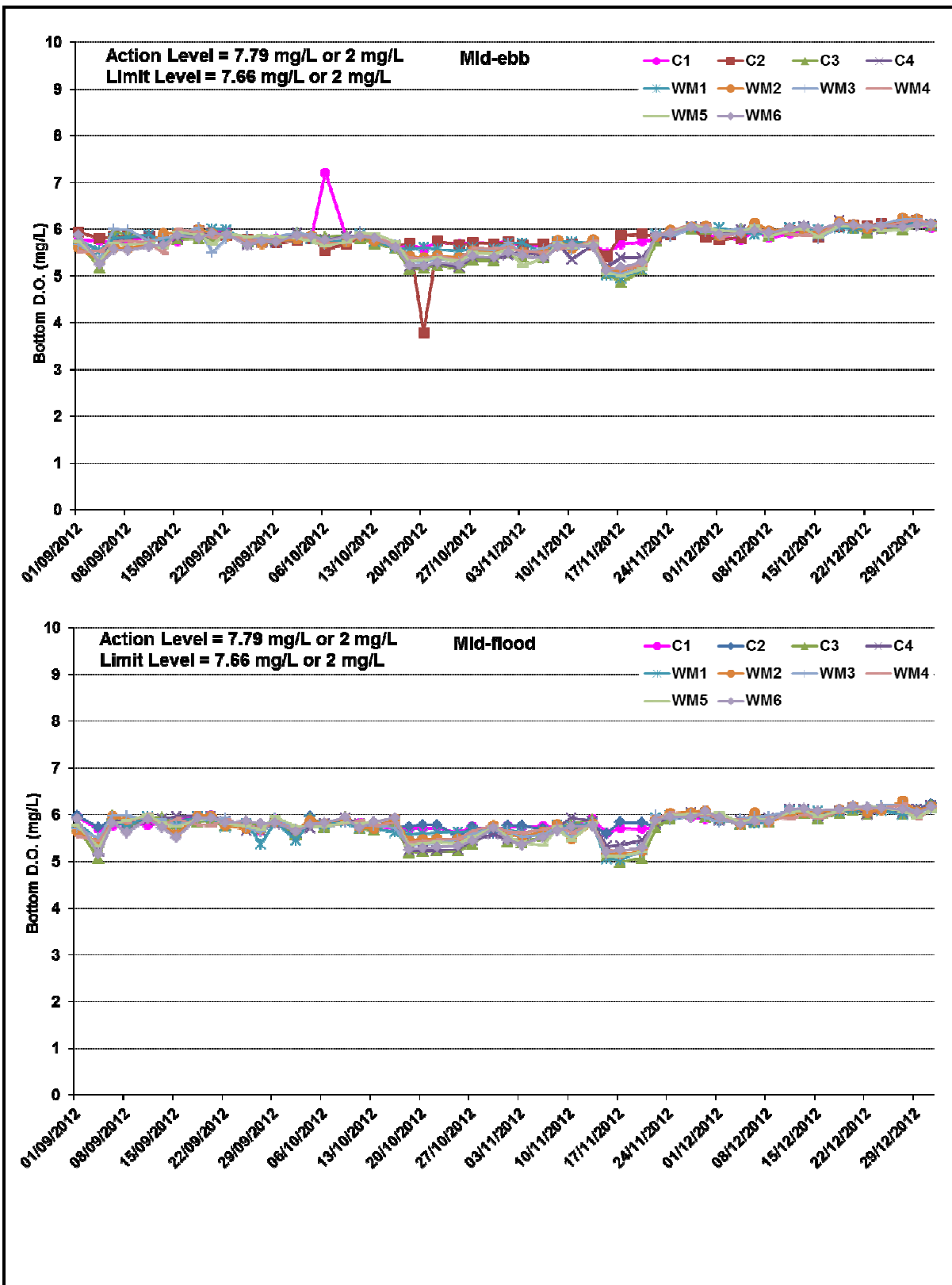
Figure B5 Impact Monitoring – Mean Level of Dissolved Oxygen (mg/L) in bottom waters between 1 September and 31 December 2012 at Monitoring Stations for Dredging Works.
