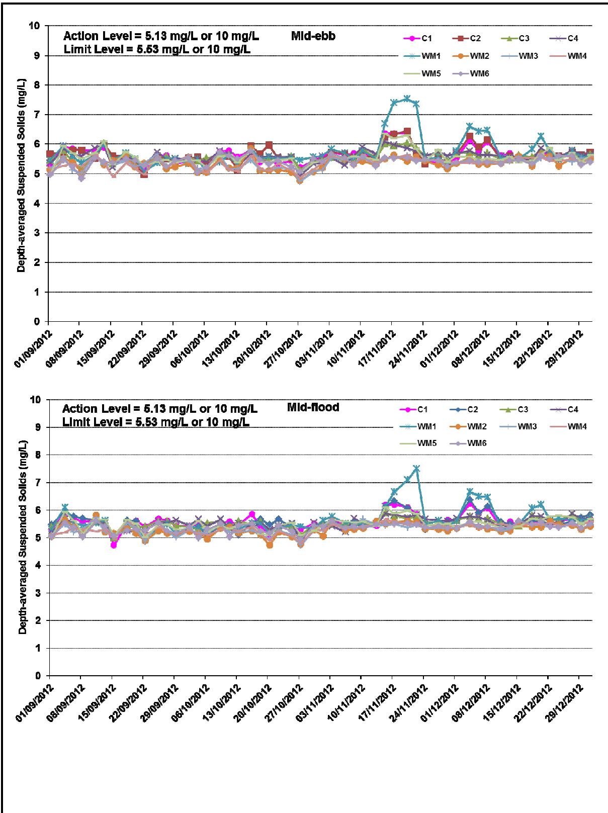
Figure B6 Impact Monitoring – Mean Depth-averaged Level of Suspended Solids (mg/L) between 1 September and 31 December 2012 at Monitoring Stations for Dredging Works.
