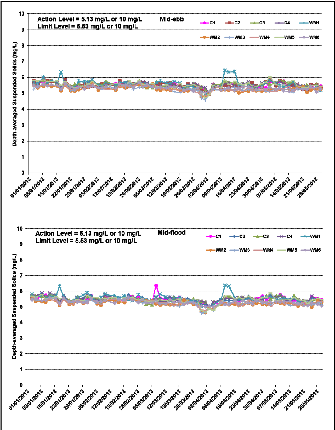
Figure B6 Impact Monitoring – Mean Depth-averaged Level of Suspended Solids (mg/L) between 3 January 2013 and 30 May 2013 at Monitoring Stations for Dredging Works.
