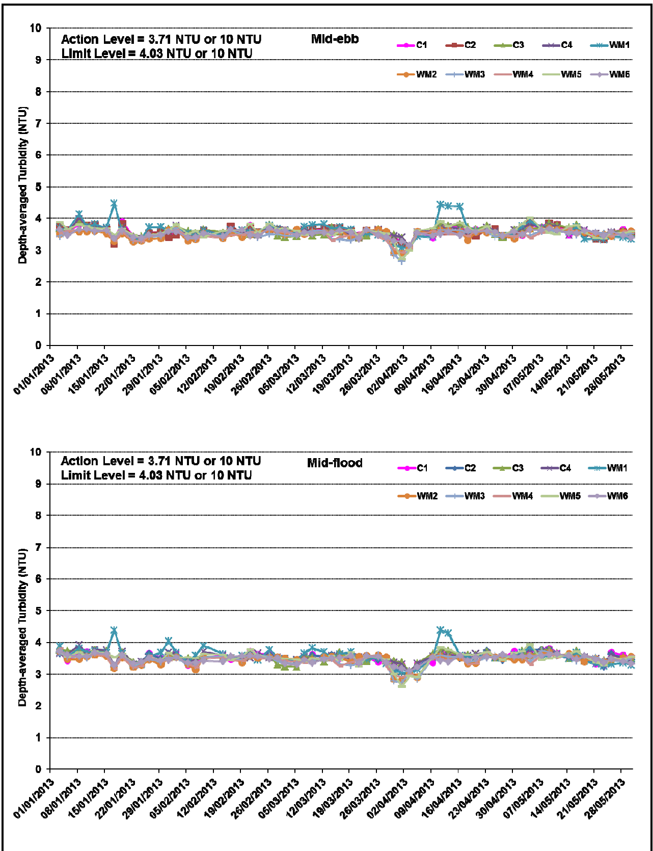
Figure B7 Impact Monitoring – Mean Depth-averaged Level of Turbidity (NTU) between 3 January 2013 and 30 May 2013 at Monitoring Stations for Dredging Works.
