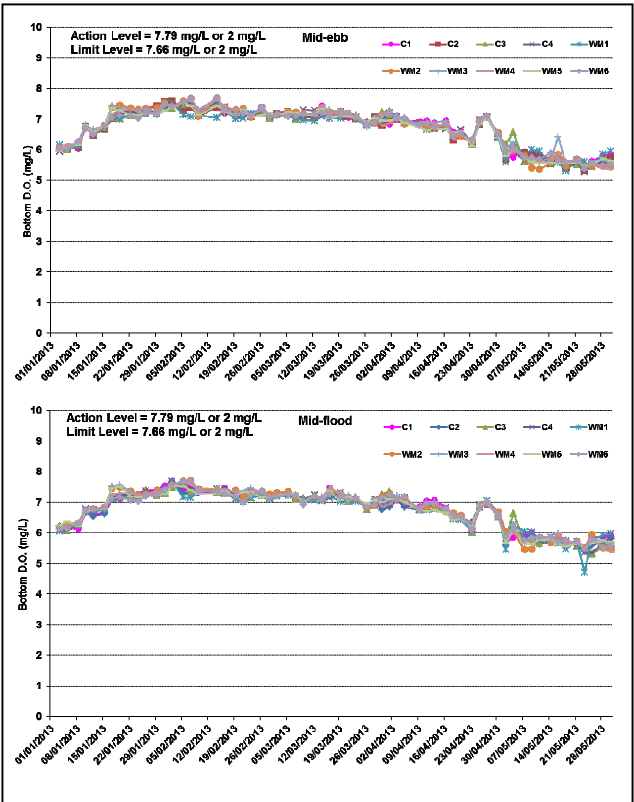
Figure B5 Impact Monitoring – Mean Level of Dissolved Oxygen (mg/L) in bottom waters between 3 January 2013 and 30 May 2013 at Monitoring Stations for Dredging Works.
