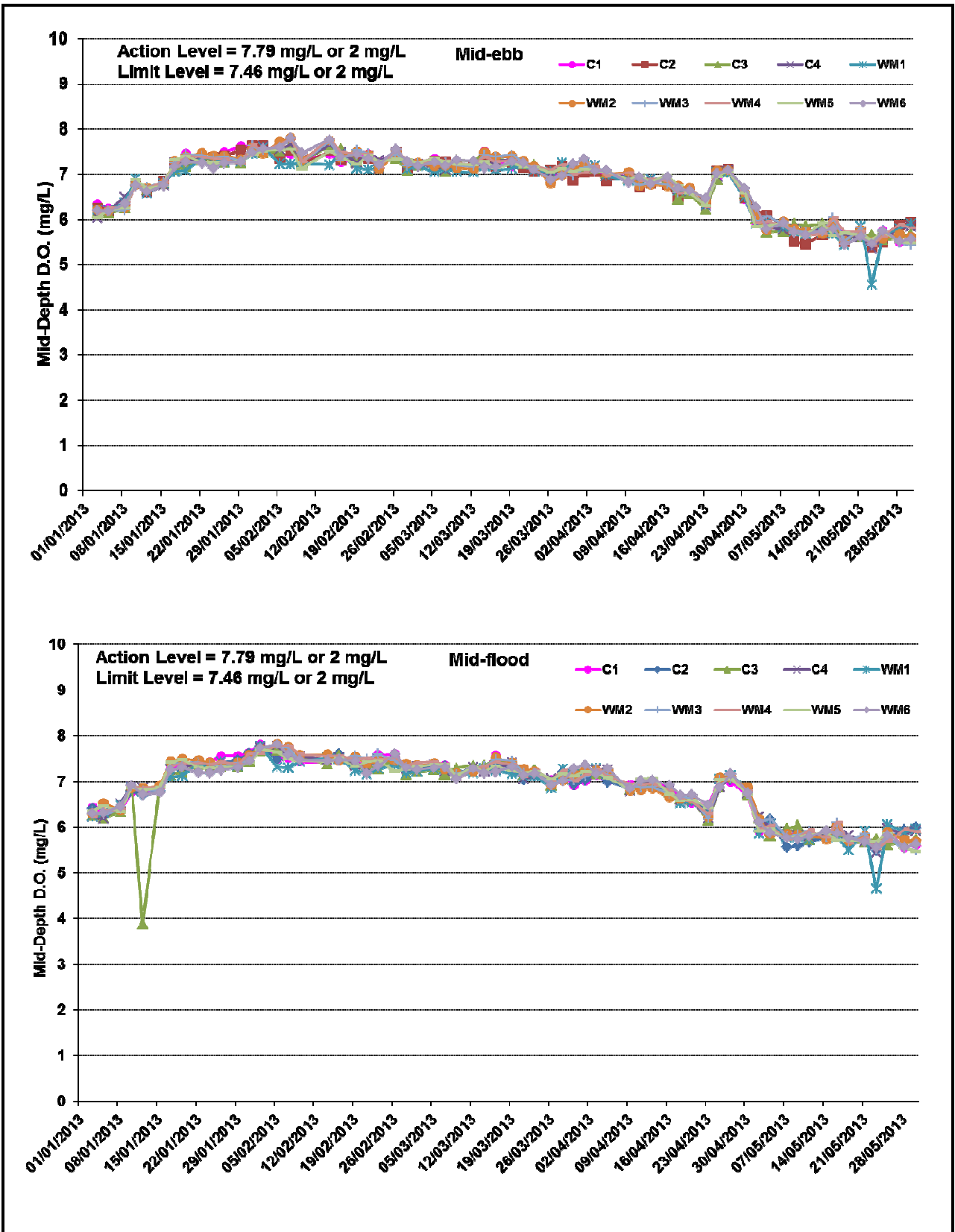
Figure B4 Impact Monitoring – Mean Level of Dissolved Oxygen (mg/L) in mid-depth waters between 3 January 2013 and 30 May 2013 at Monitoring Stations for Dredging Works.
