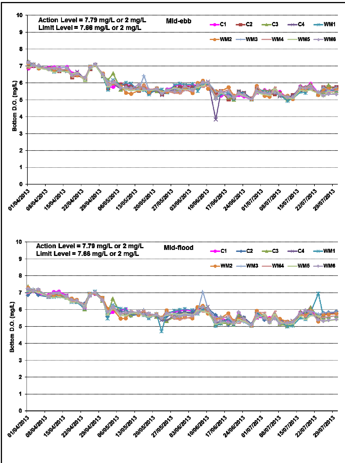
Figure B5 Impact Monitoring – Mean Level of Dissolved Oxygen (mg/L) in bottom waters between 1 April 2013 and 30 July 2013 at Monitoring Stations for Marine Works.
