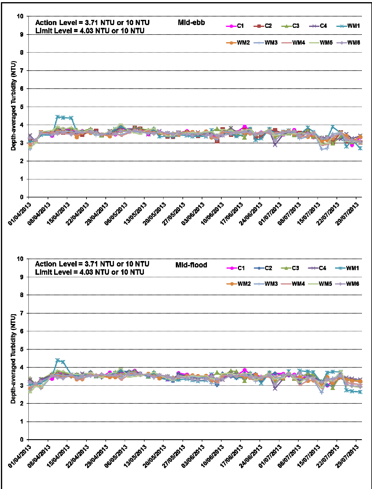
Figure B7 Impact Monitoring – Mean Depth-averaged Level of Turbidity (NTU) between 1 April 2013 and 30 July 2013 at Monitoring Stations for Marine Works.
