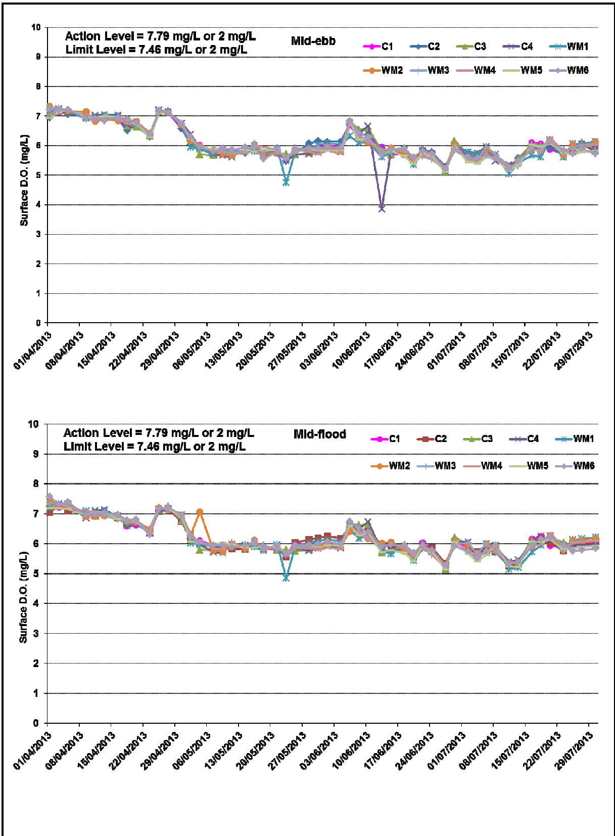
Figure B3 Impact Monitoring – Mean Level of Dissolved Oxygen (mg/L) in surface waters between 1 April 2013 and 30 July 2013 at Monitoring Stations for Marine Works.
