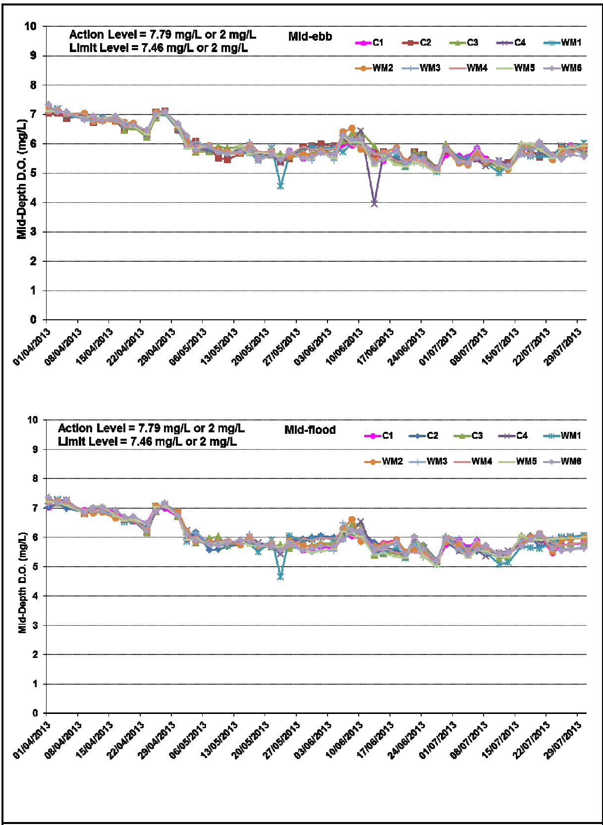
Figure B4 Impact Monitoring – Mean Level of Dissolved Oxygen (mg/L) in mid-depth waters between 1 April 2013 and 30 July 2013 at Monitoring Stations for Marine Works.
