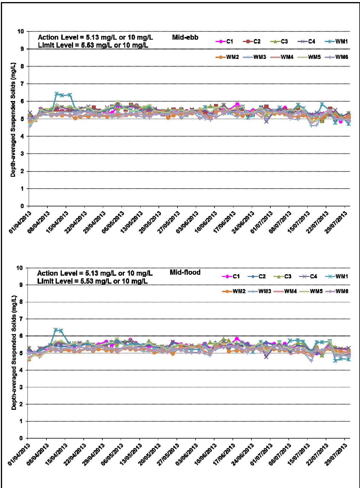
Figure B6 Impact Monitoring – Mean Depth-averaged Level of Suspended Solids (mg/L) between 1 April 2013 and 30 July 2013 at Monitoring Stations for Marine Works.
