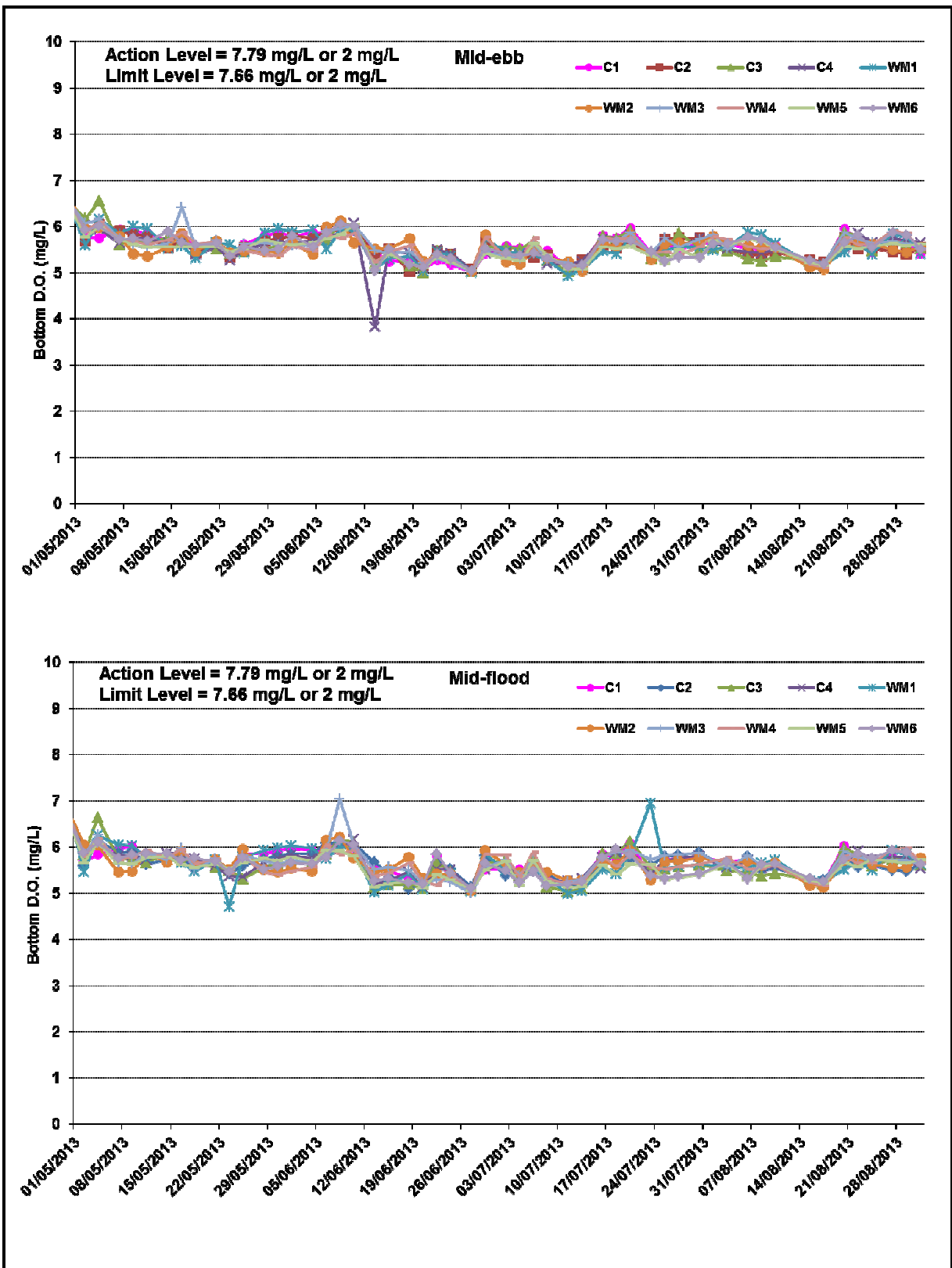
Figure B5 Impact Monitoring – Mean Level of Dissolved Oxygen (mg/L) in bottom waters between 1 May 2013 and 31 August 2013 at Monitoring Stations for Marine Works.
