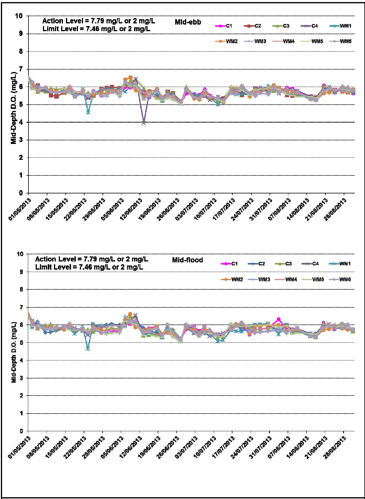
Figure B4 Impact Monitoring – Mean Level of Dissolved Oxygen (mg/L) in mid-depth waters between 1 May 2013 and 31 August 2013 at Monitoring Stations for Marine Works.
