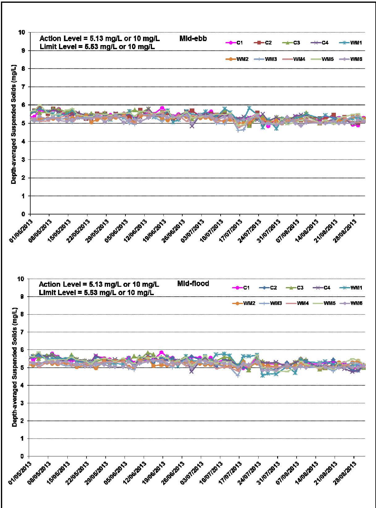
Figure B6 Impact Monitoring – Mean Depth-averaged Level of Suspended Solids (mg/L) between 1 May 2013 and 31 August 2013 at Monitoring Stations for Marine Works.
