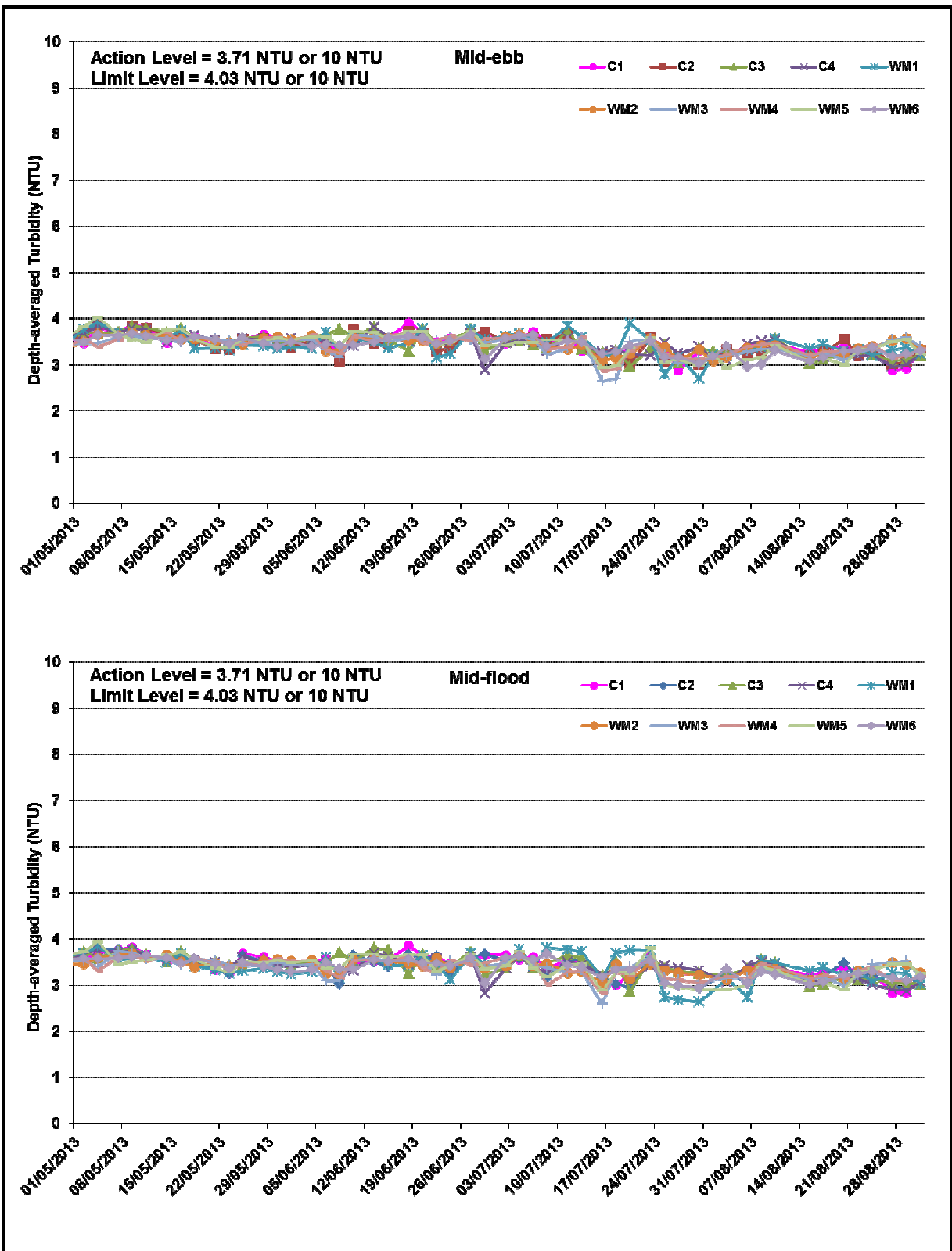
Figure B7 Impact Monitoring – Mean Depth-averaged Level of Turbidity (NTU) between 1 May 2013 and 31 August 2013 at Monitoring Stations for Marine Works.
