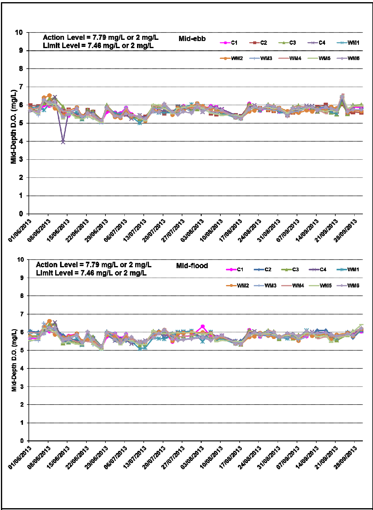
Figure B4 Impact Monitoring – Mean Level of Dissolved Oxygen (mg/L) in mid-depth waters between 1 June 2013 and 30 September 2013 at Monitoring Stations for Marine Works.
