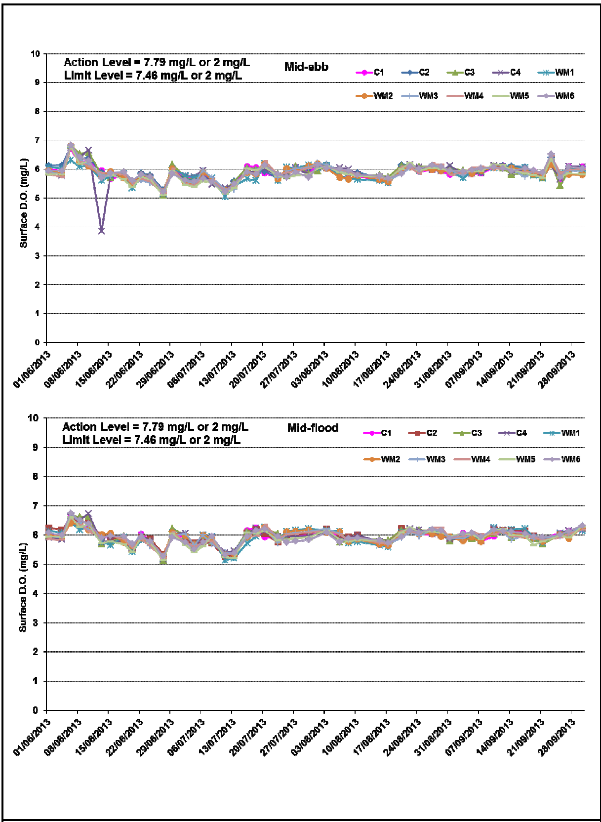
Figure B3 Impact Monitoring – Mean Level of Dissolved Oxygen (mg/L) in surface waters between 1 June 2013 and 30 September 2013 at Monitoring Stations for Marine Works.
