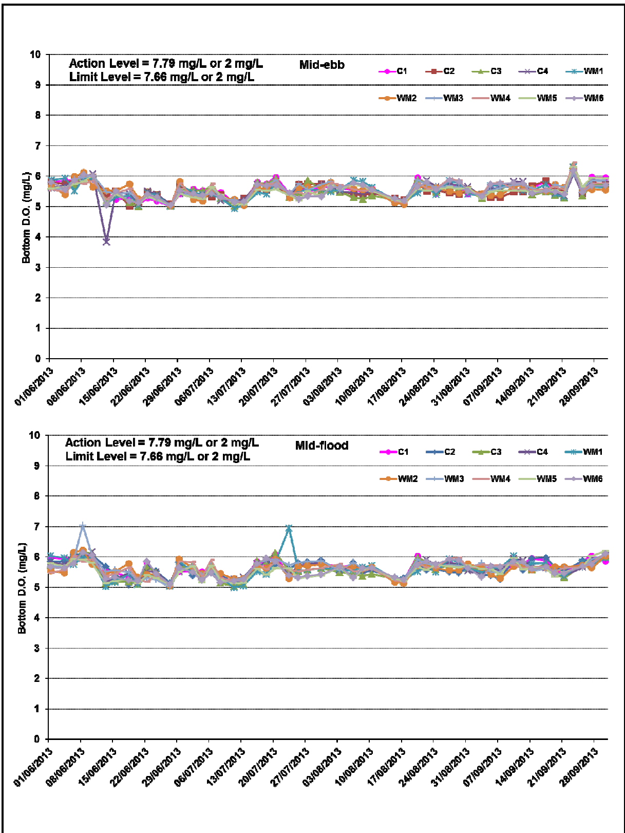
Figure B5 Impact Monitoring – Mean Level of Dissolved Oxygen (mg/L) in bottom waters between 1 June 2013 and 30 September 2013 at Monitoring Stations for Marine Works.
