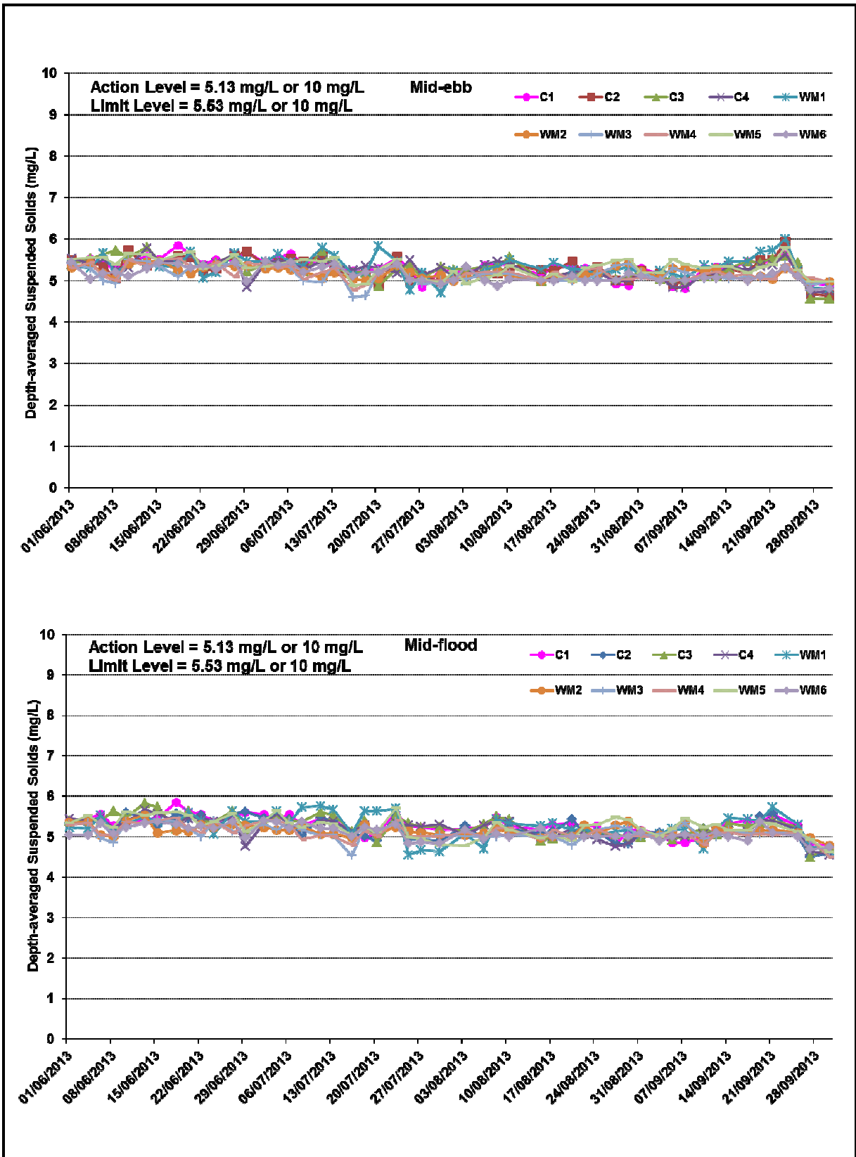
Figure B6 Impact Monitoring – Mean Depth-averaged Level of Suspended Solids (mg/L) between 1 June 2013 and 30 September 2013 at Monitoring Stations for Marine Works.
