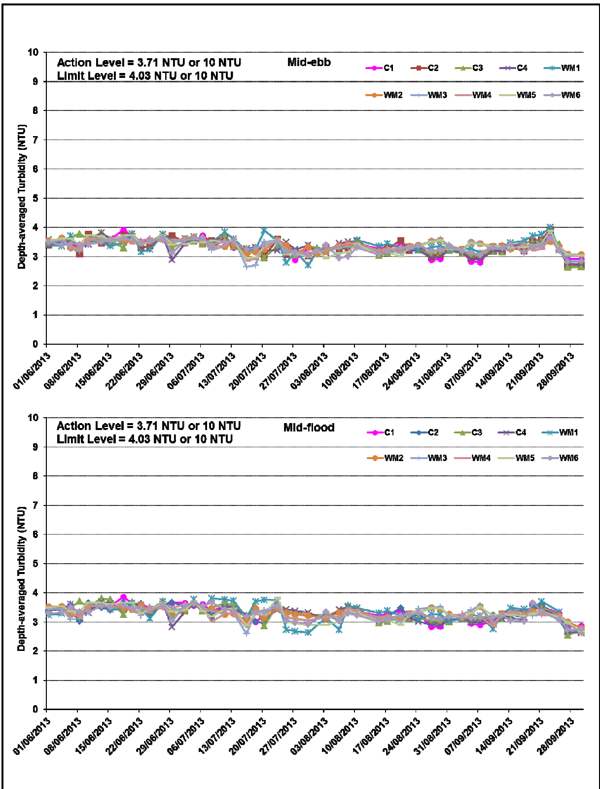
Figure B7 Impact Monitoring – Mean Depth-averaged Level of Turbidity (NTU) between 1 June 2013 and 30 September 2013 at Monitoring Stations for Marine Works.
