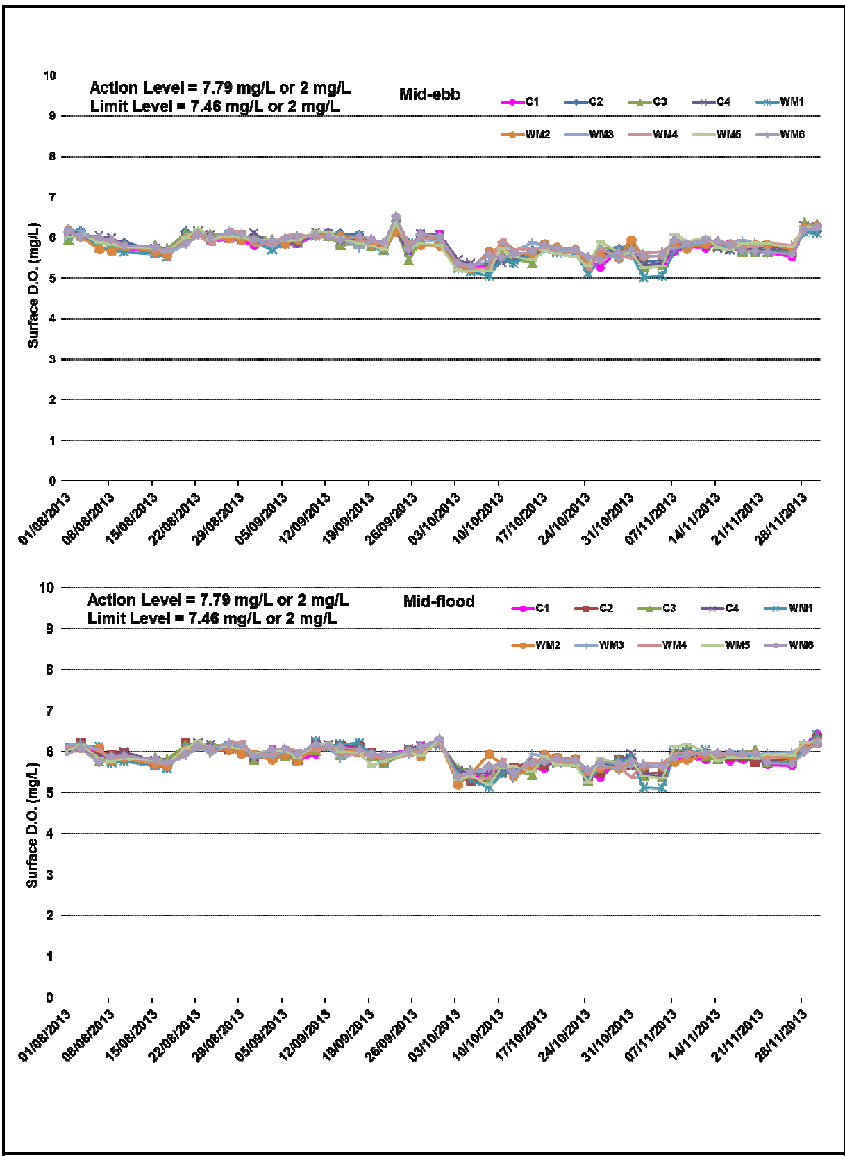
Figure B3 Impact Monitoring – Mean Level of Dissolved Oxygen (mg/L) in surface waters between 1 August 2013 and 30 November 2013 at Monitoring Stations for Marine Works.
