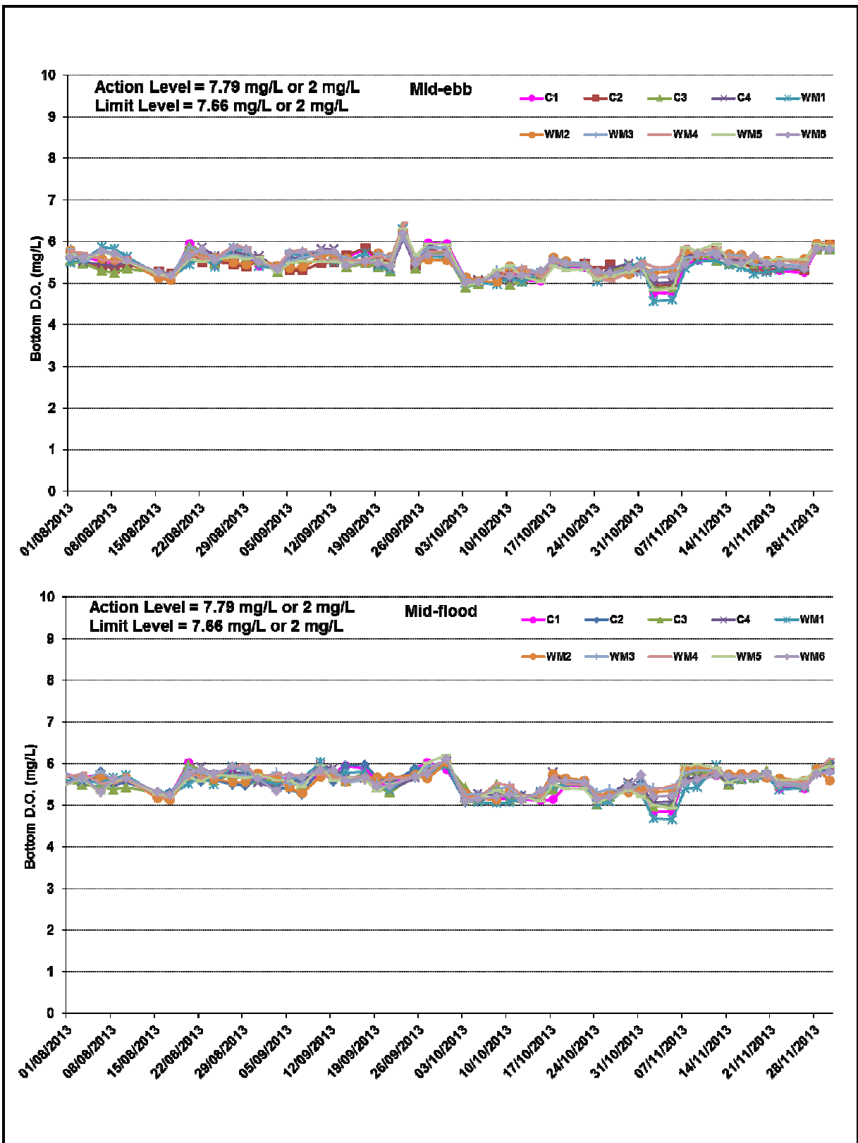
Figure B5 Impact Monitoring – Mean Level of Dissolved Oxygen (mg/L) in bottom waters between 1 August 2013 and 30 November 2013 at Monitoring Stations for Marine Works.
