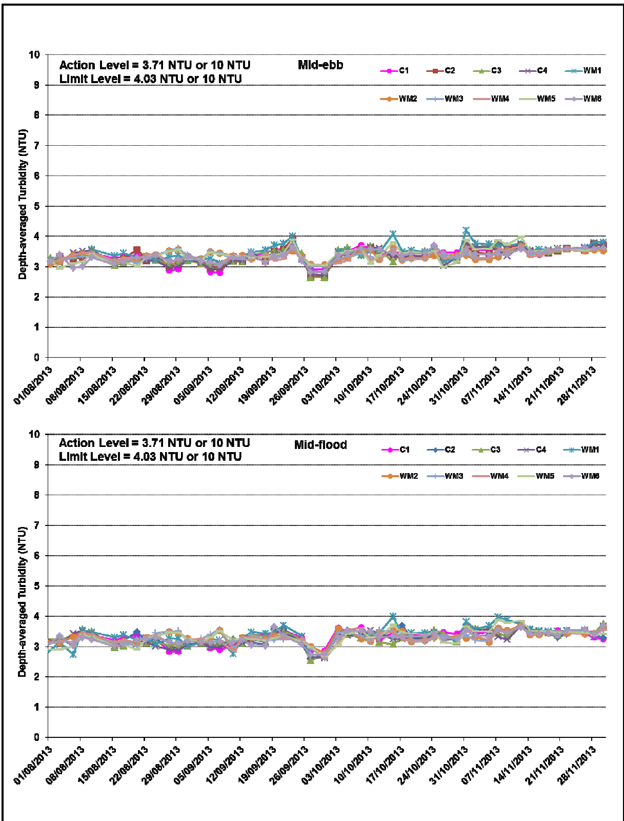
Figure B7 Impact Monitoring – Mean Depth-averaged Level of Turbidity (NTU) between 1 August 2013 and 30 November 2013 at Monitoring Stations for Marine Works.
