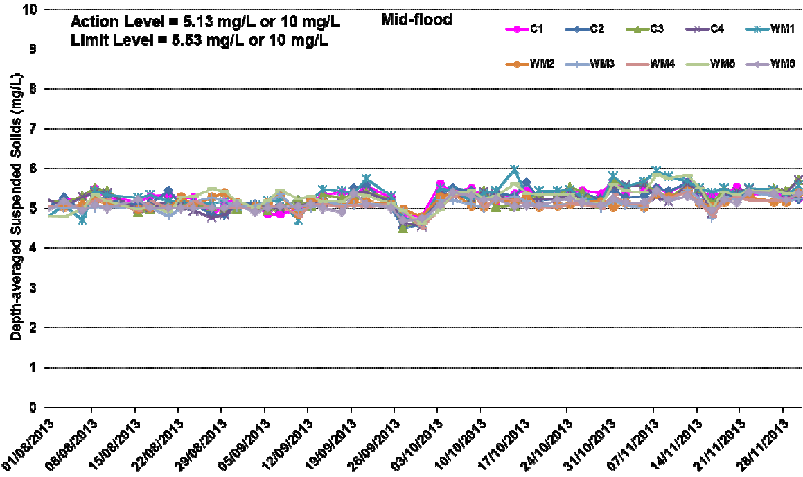
Figure B6 Impact Monitoring – Mean Depth-averaged Level of Suspended Solids (mg/L) between 1 August 2013 and 30 November 2013 at Monitoring Stations for Marine Works.
