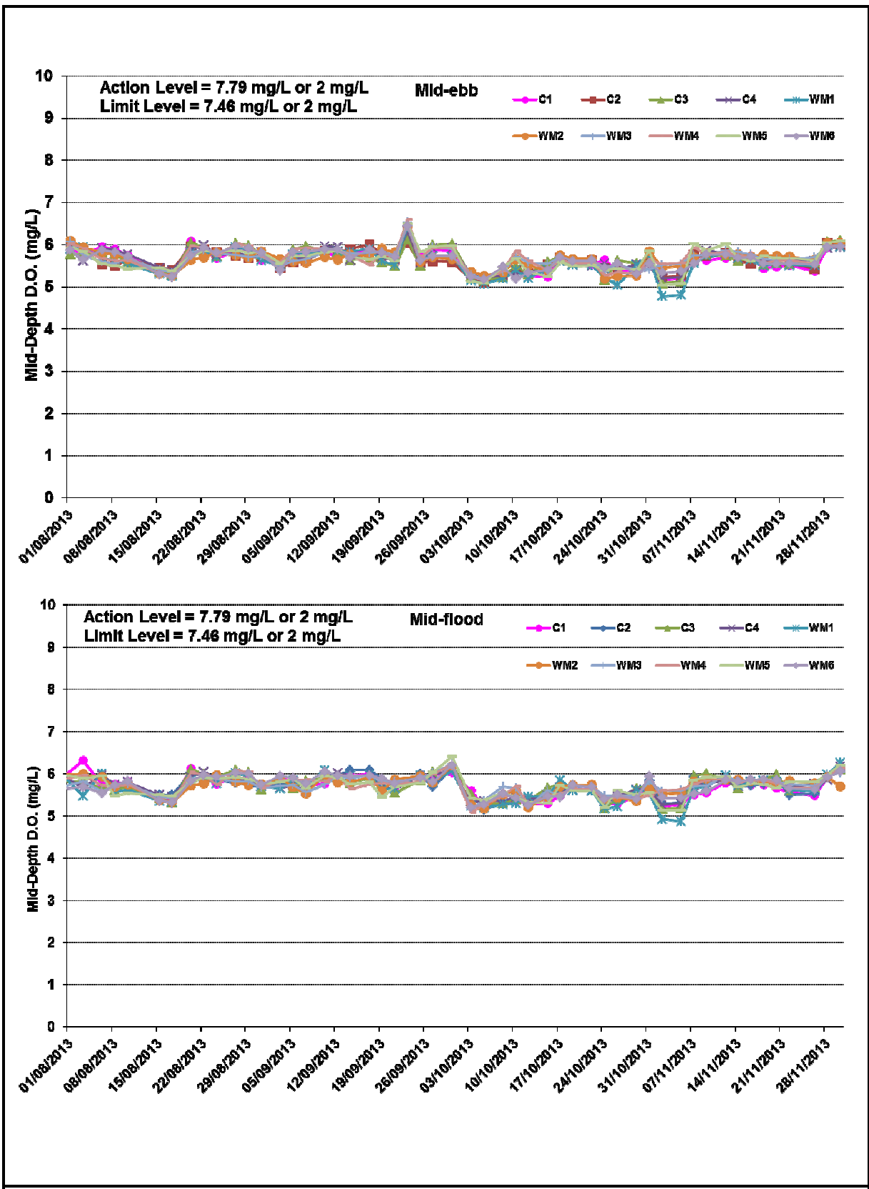
Figure B4 Impact Monitoring – Mean Level of Dissolved Oxygen (mg/L) in mid-depth waters between 1 August 2013 and 30 November 2013 at Monitoring Stations for Marine Works.
