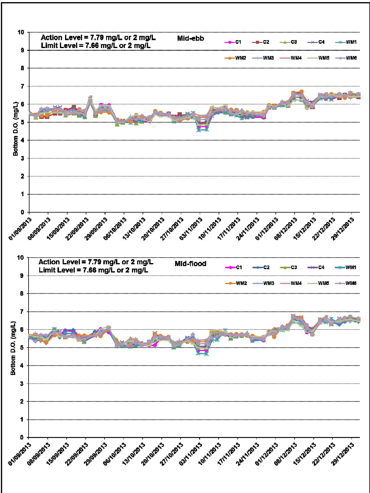
Figure B5 Impact Monitoring – Mean Level of Dissolved Oxygen (mg/L) in bottom waters between 1 September and 31 December 2013 at Monitoring Stations for Marine Works.
