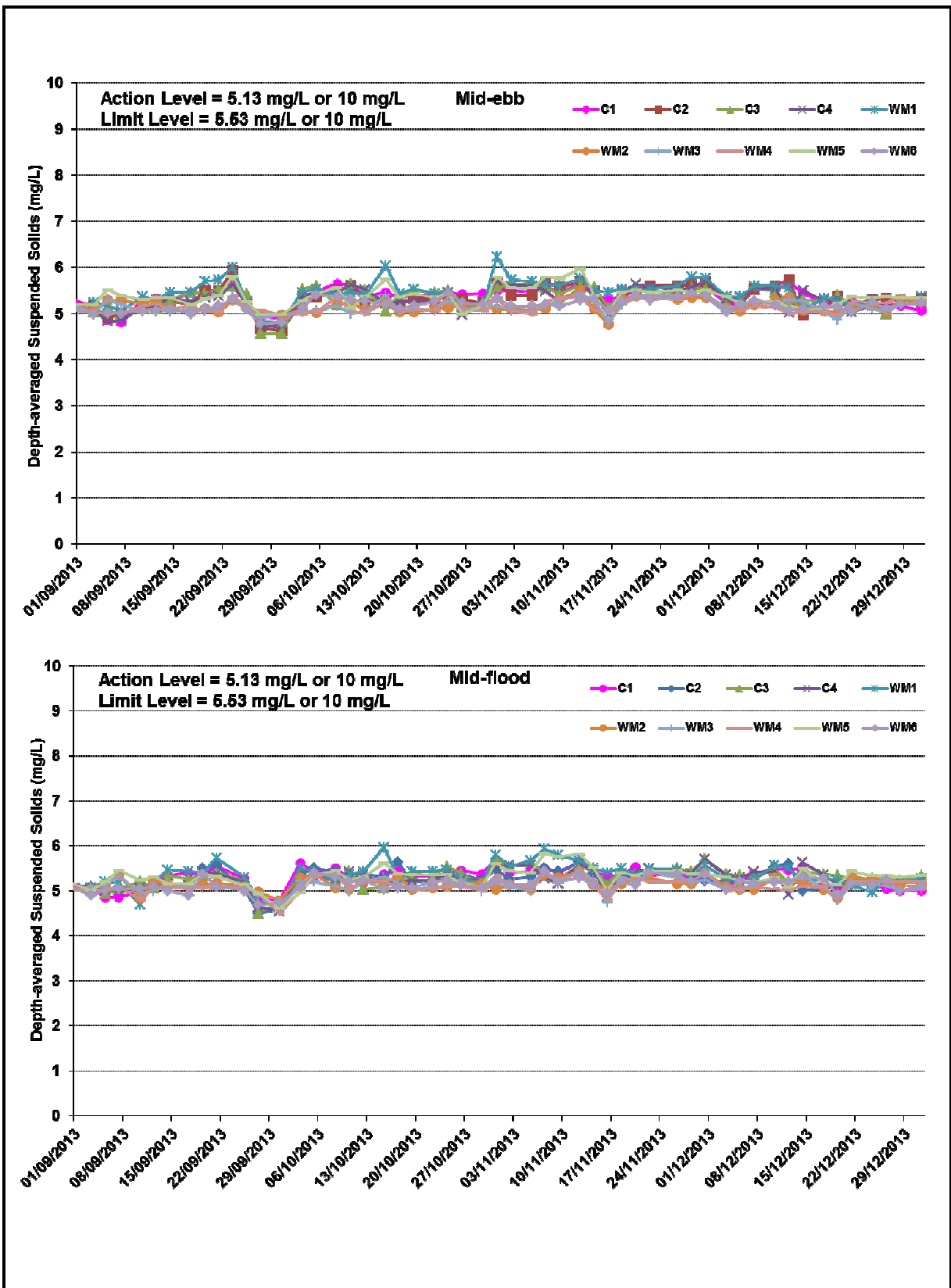
Figure B6 Impact Monitoring – Mean Depth-averaged Level of Suspended Solids (mg/L) between 1 September and 31 December 2013 at Monitoring Stations for Marine Works.
