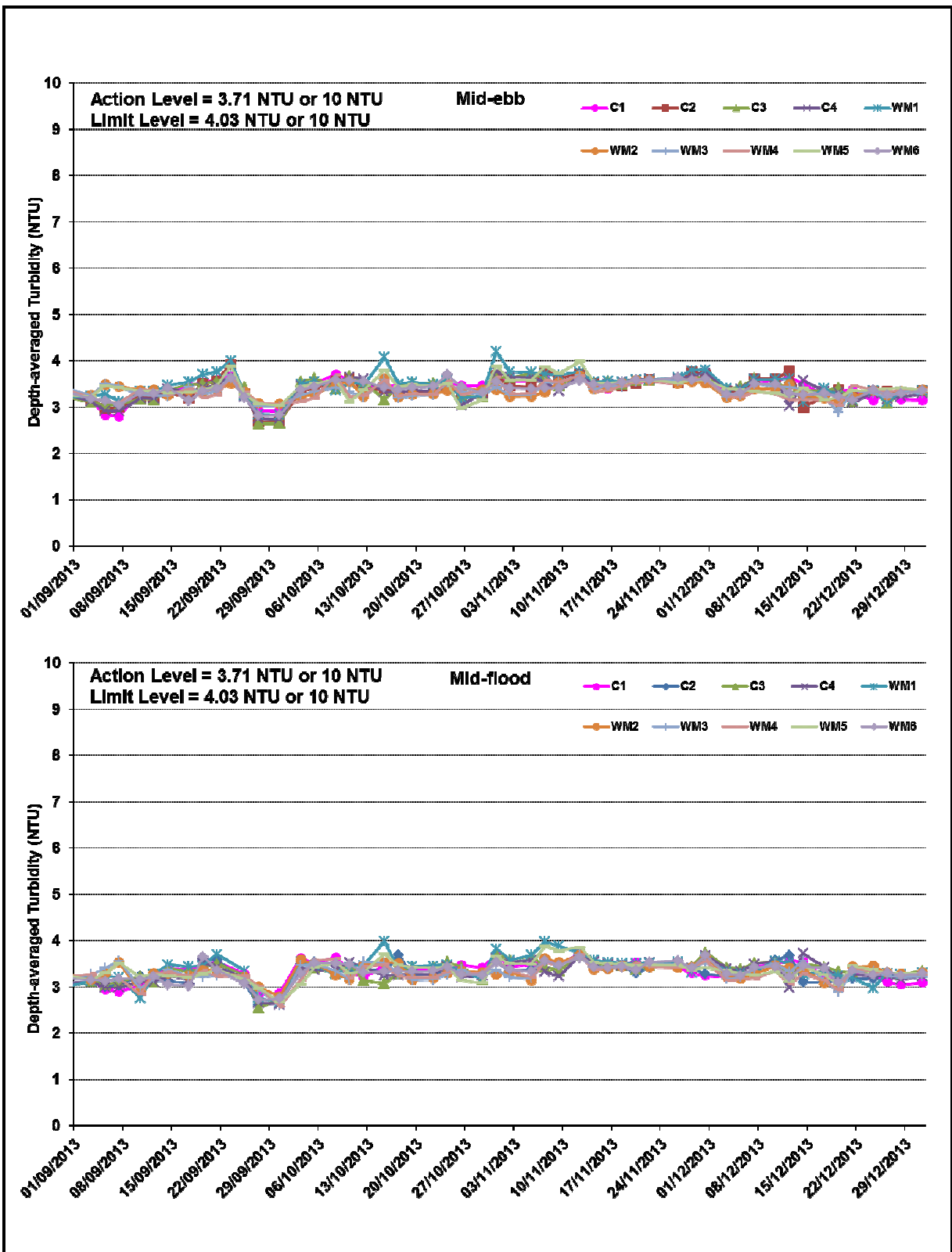
Figure B7 Impact Monitoring – Mean Depth-averaged Level of Turbidity (NTU) between 1 September and 31 December 2013 at Monitoring Stations for Marine Works.
