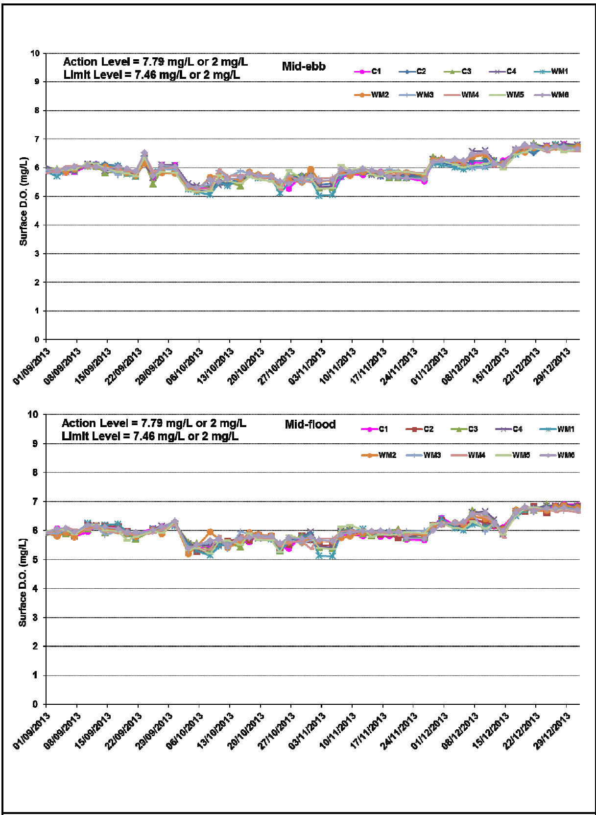
Figure B3 Impact Monitoring – Mean Level of Dissolved Oxygen (mg/L) in surface waters between 1 September and 31 December 2013 at Monitoring Stations for Marine Works.
