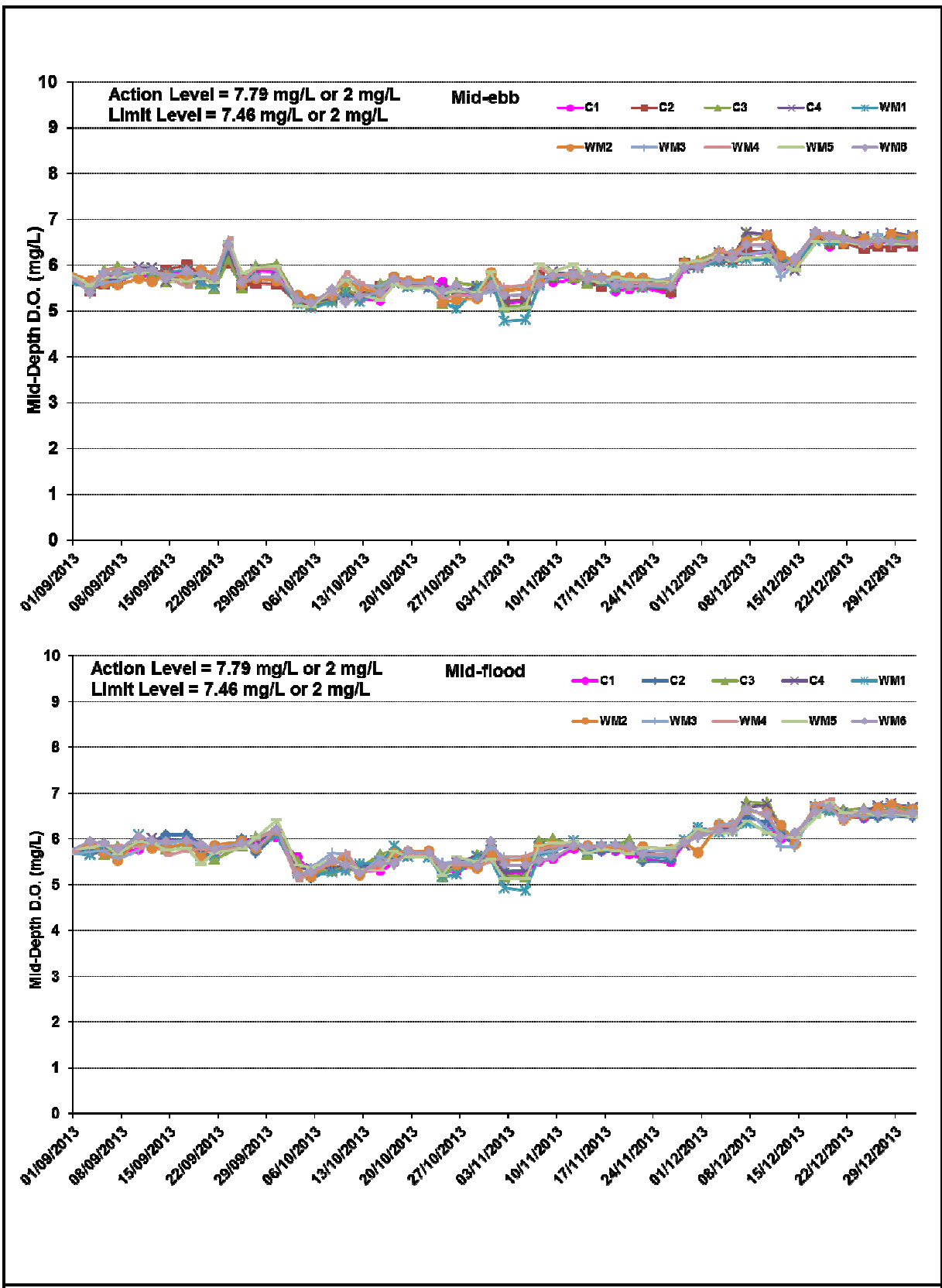
Figure B4 Impact Monitoring – Mean Level of Dissolved Oxygen (mg/L) in mid-depth waters between 1 September and 31 December 2013 at Monitoring Stations for Marine Works.
