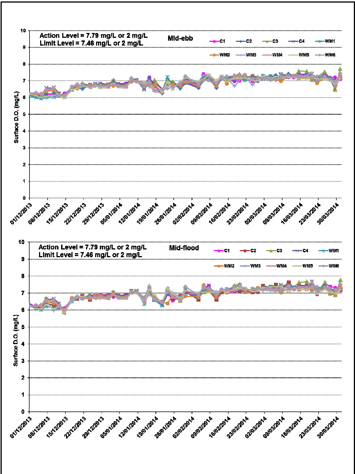
Figure B3 Impact Monitoring – Mean Level of Dissolved Oxygen (mg/L) in surface waters between 1 December 2013 and 31 March 2014 at Monitoring Stations for Marine Works.
