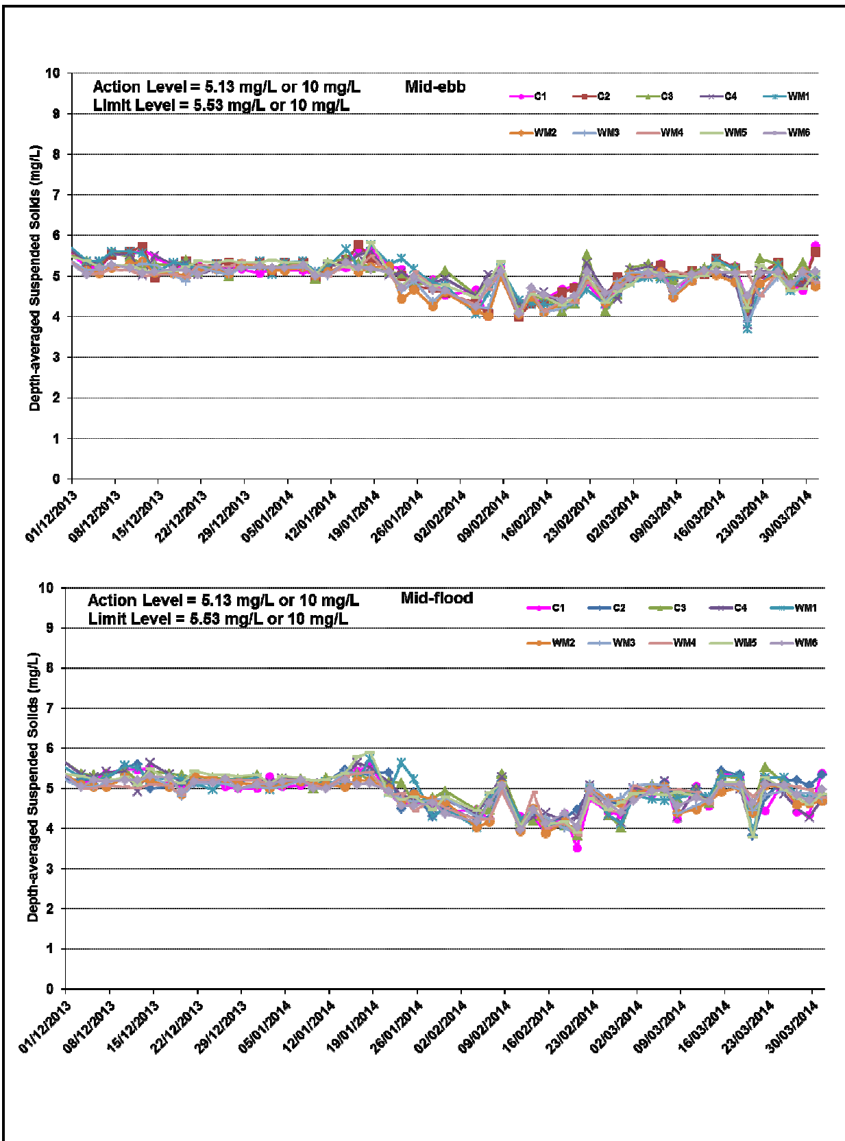
Figure B6 Impact Monitoring – Mean Depth-averaged Level of Suspended Solids (mg/L) between 1 December 2013 and 31 March 2014 at Monitoring Stations for Marine Works.
