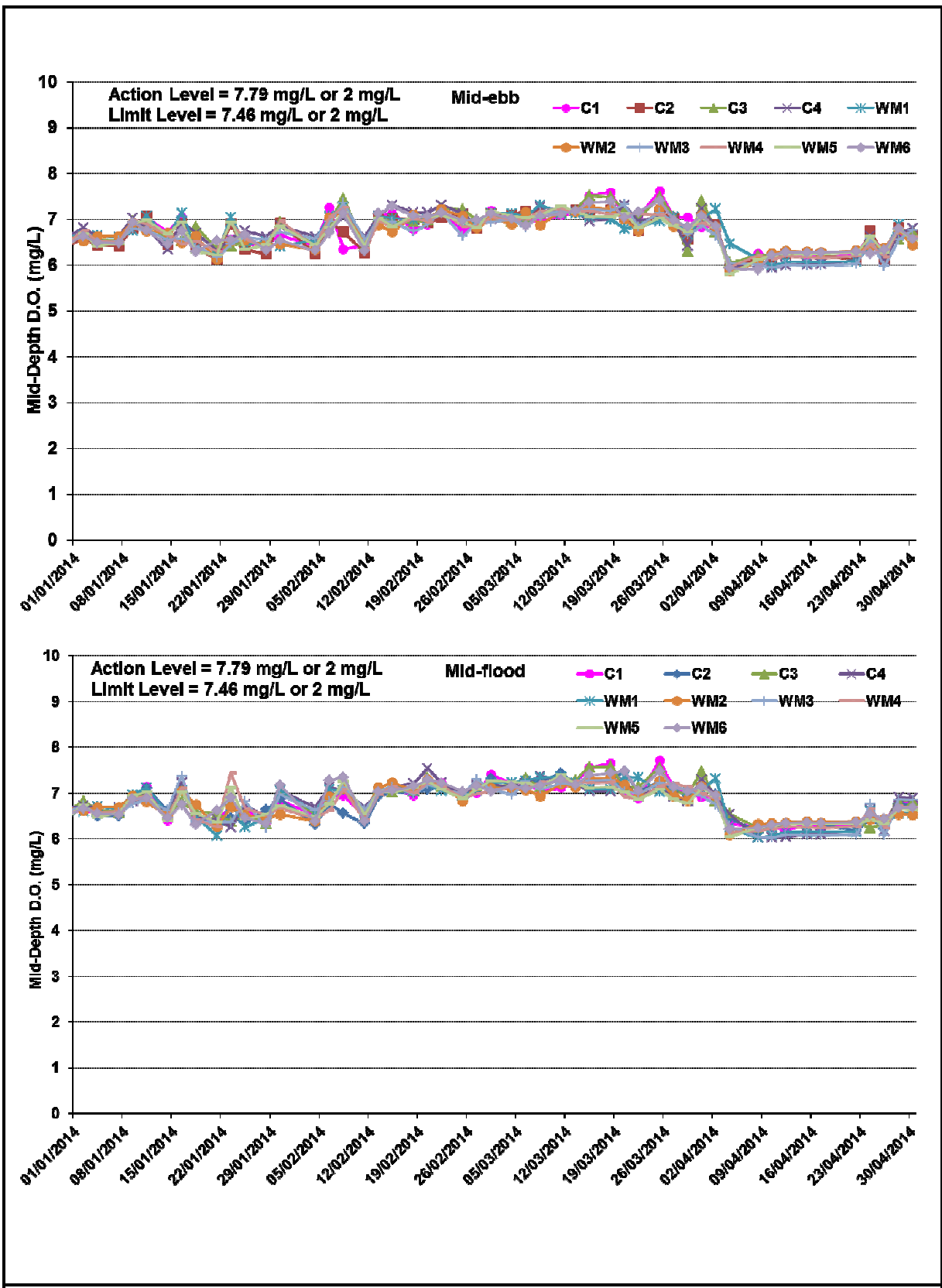
Figure B4 Impact Monitoring – Mean Level of Dissolved Oxygen (mg/L) in mid-depth waters between 1 January 2014 and 30 April 2014 at Monitoring Stations for Marine Works.
