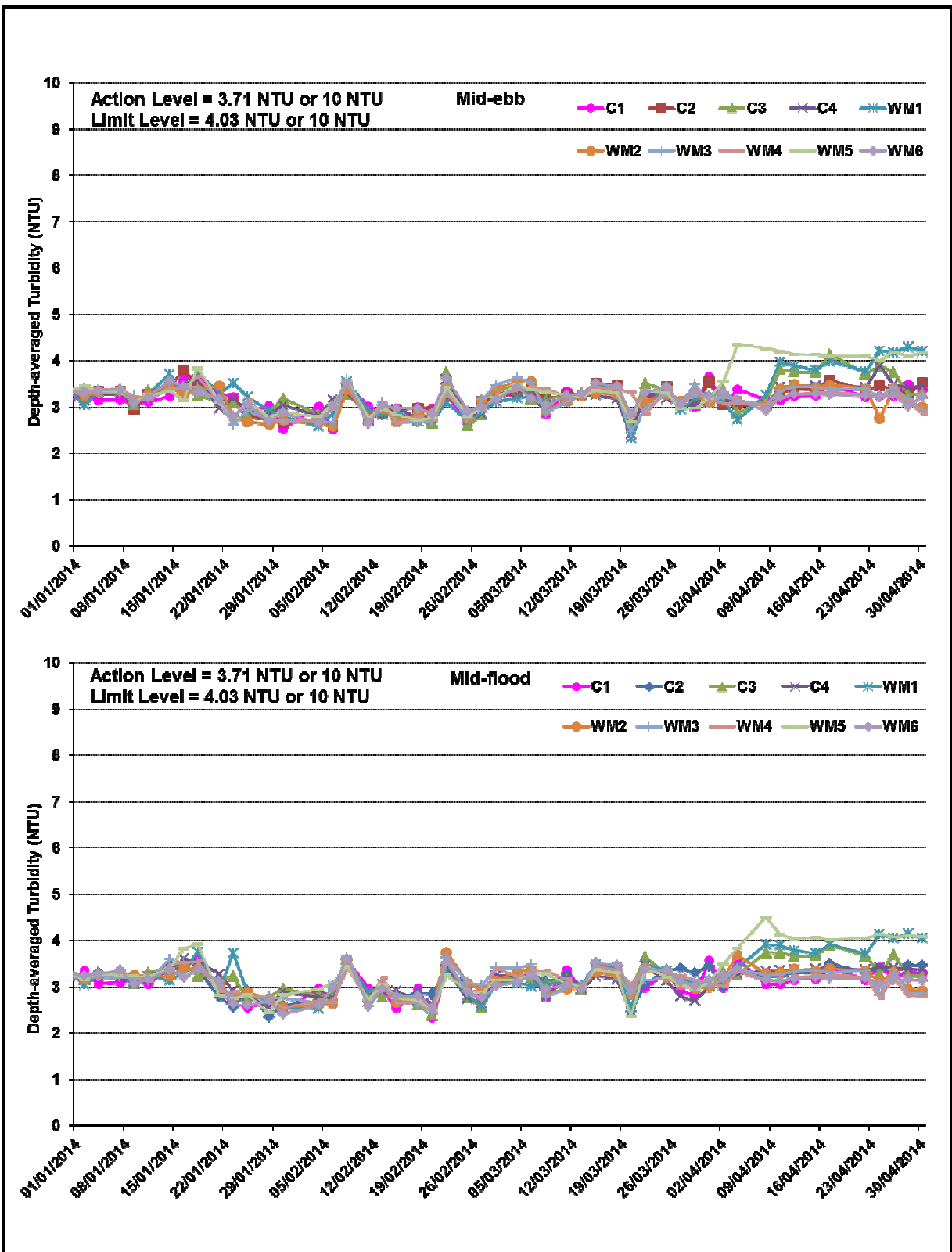
Figure B7 Impact Monitoring – Mean Depth-averaged Level of Turbidity (NTU) between 1 January 2014 and 30 April 2014 at Monitoring Stations for Marine Works.
