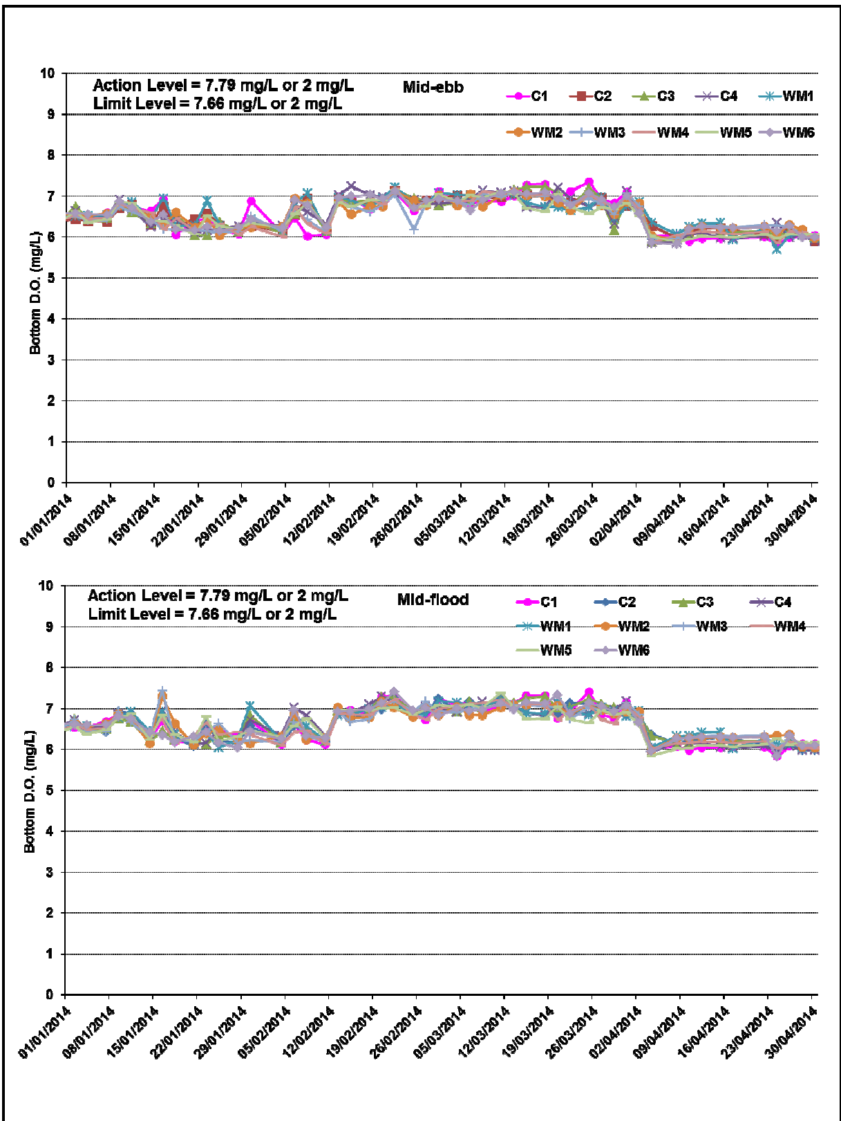
Figure B5 Impact Monitoring – Mean Level of Dissolved Oxygen (mg/L) in bottom waters between 1 January 2014 and 30 April 2014 at Monitoring Stations for Marine Works.
