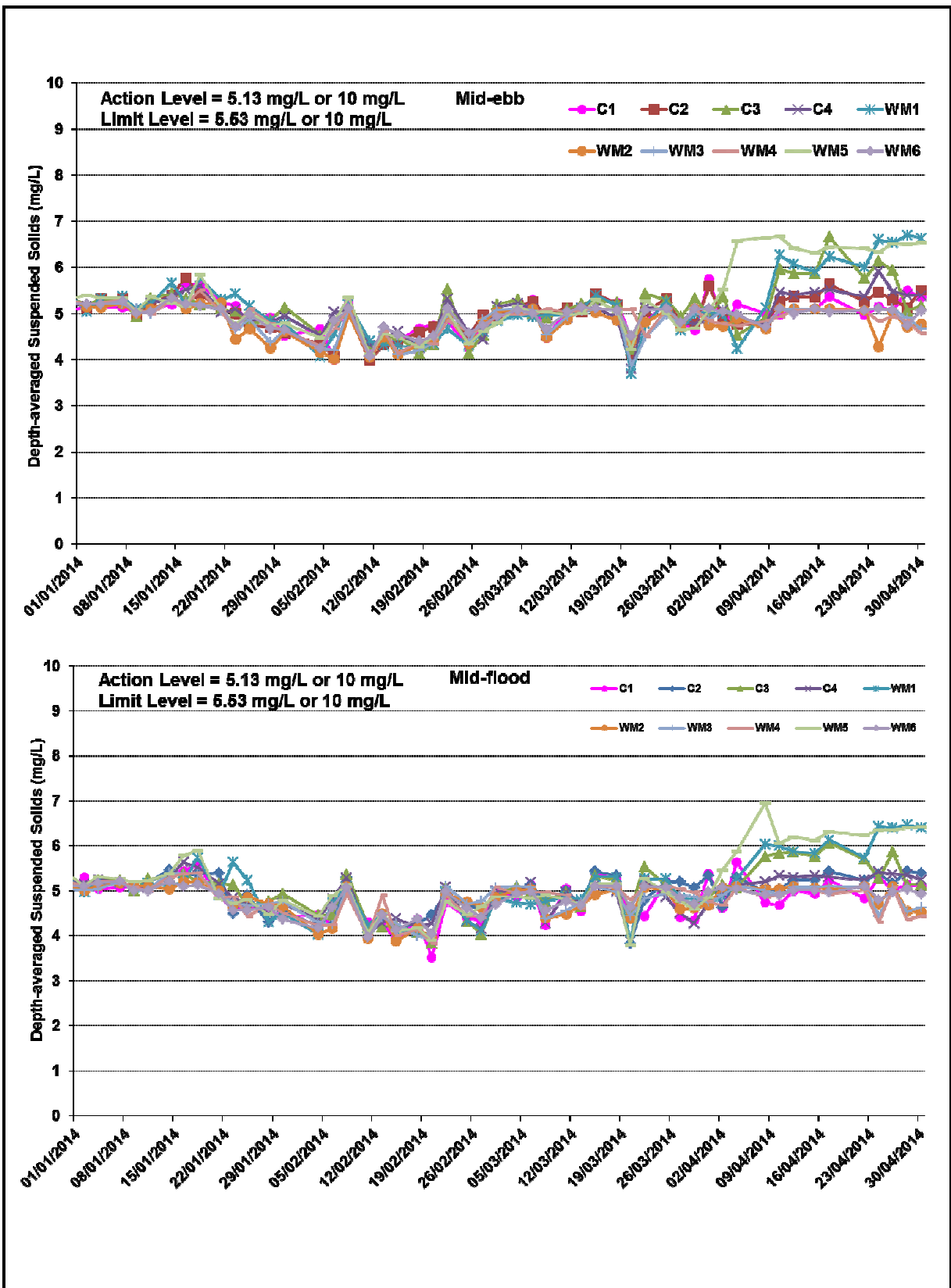
Figure B6 Impact Monitoring – Mean Depth-averaged Level of Suspended Solids (mg/L) between 1 January 2014 and 30 April 2014 at Monitoring Stations for Marine Works.
