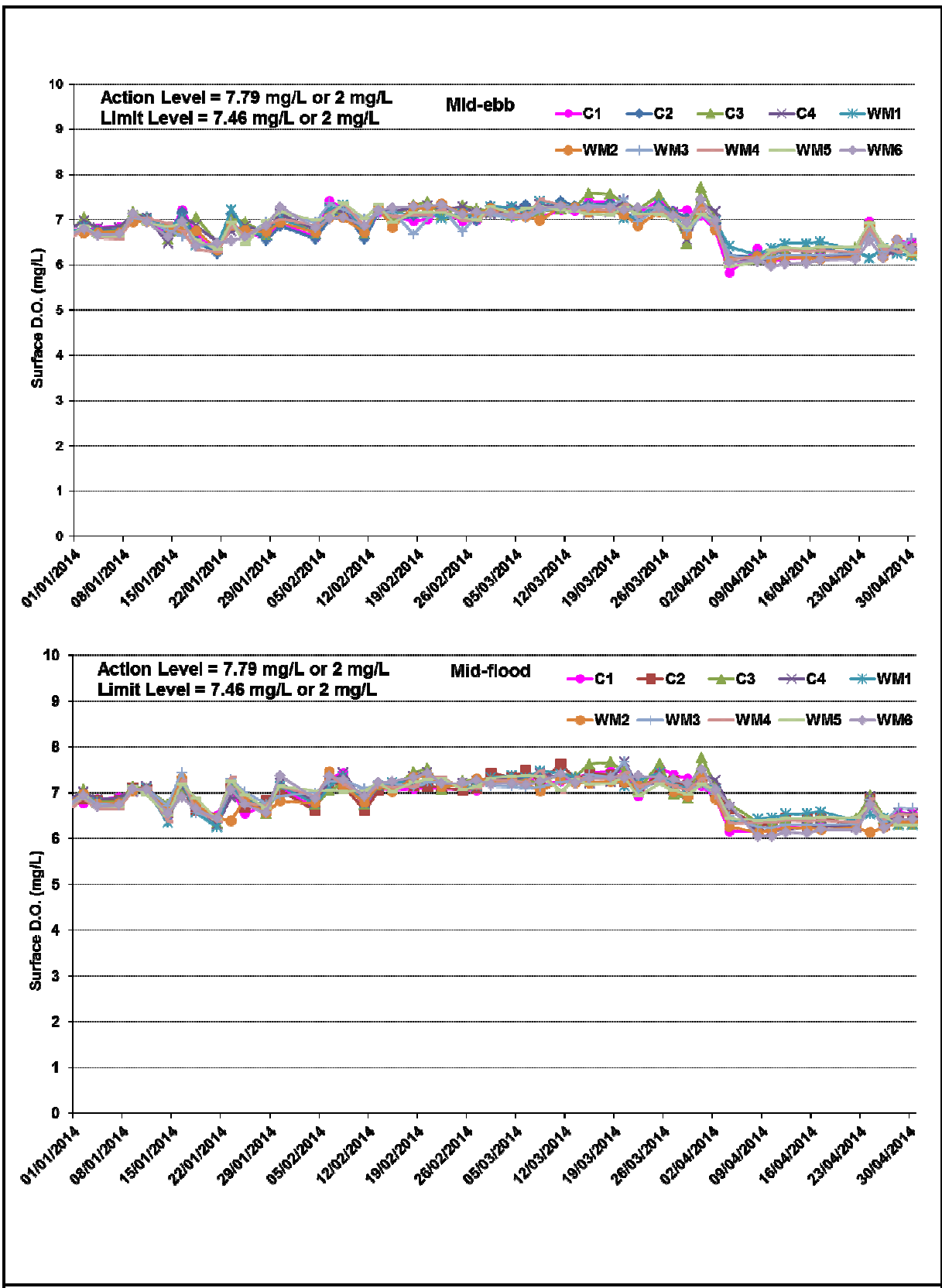
Figure B3 Impact Monitoring – Mean Level of Dissolved Oxygen (mg/L) in surface waters between 1 January 2014 and 30 April 2014 at Monitoring Stations for Marine Works.
