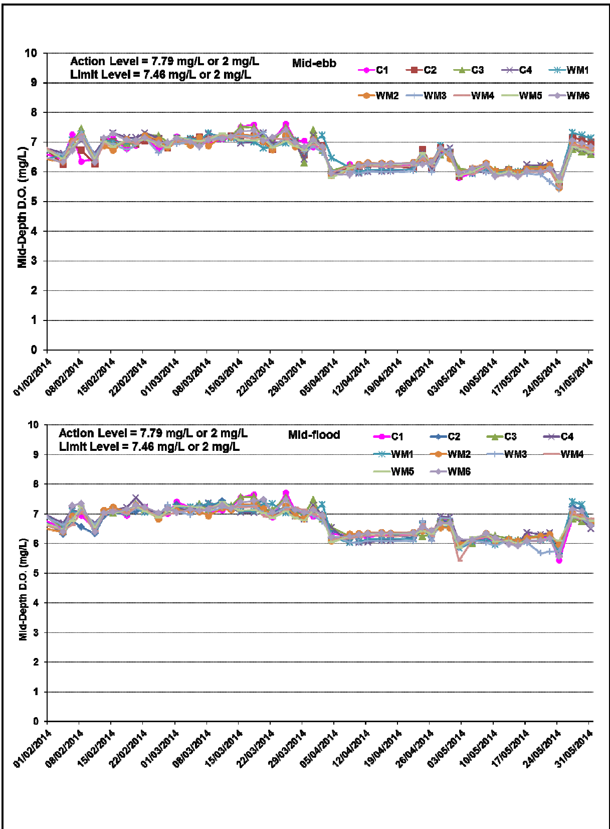
Figure B4 Impact Monitoring – Mean Level of Dissolved Oxygen (mg/L) in mid-depth waters between 1 February 2014 and 31 May 2014 at Monitoring Stations for Marine Works.
