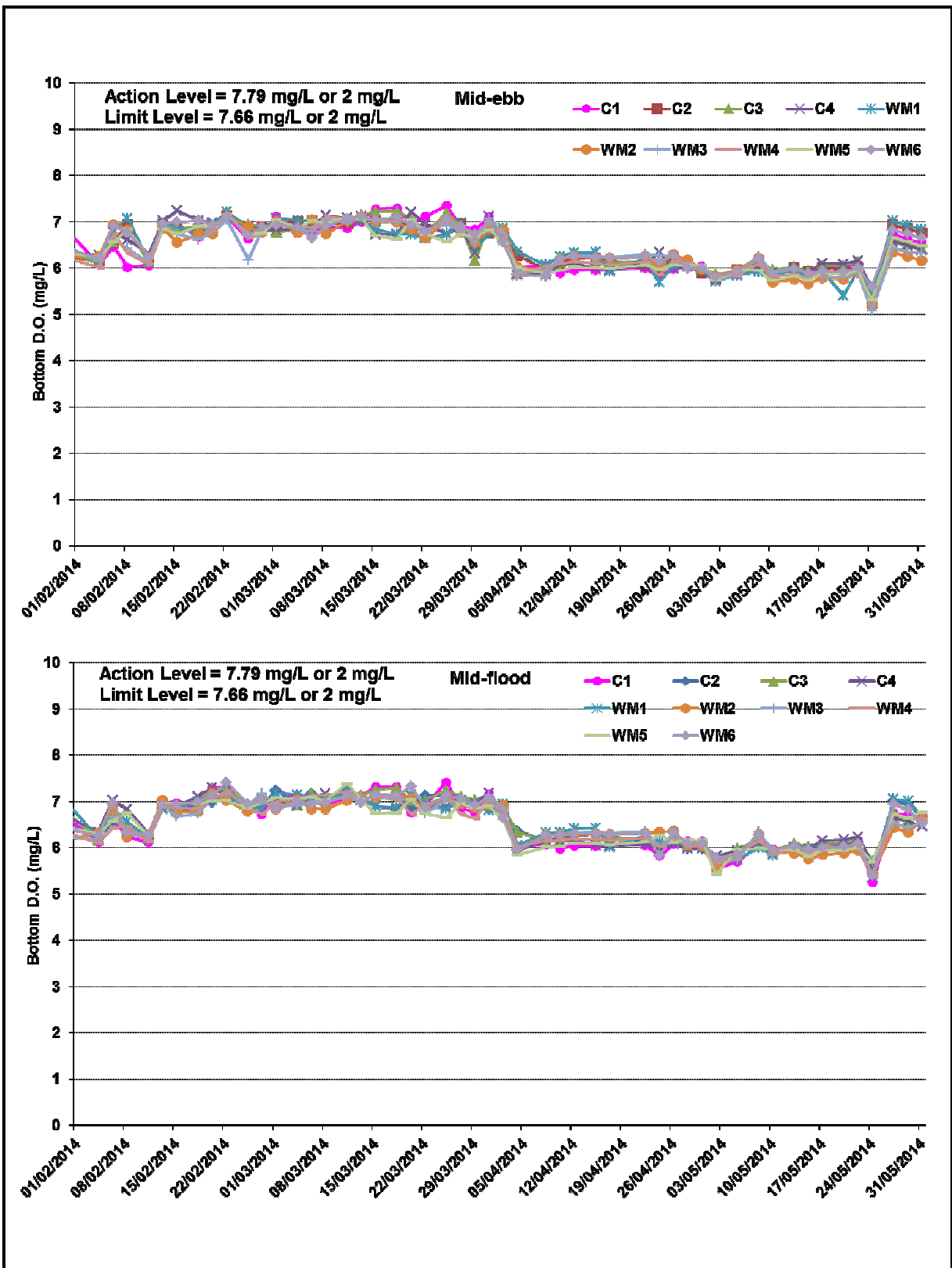
Figure B5 Impact Monitoring – Mean Level of Dissolved Oxygen (mg/L) in bottom waters between 1 February 2014 and 31 May 2014 at Monitoring Stations for Marine Works.
