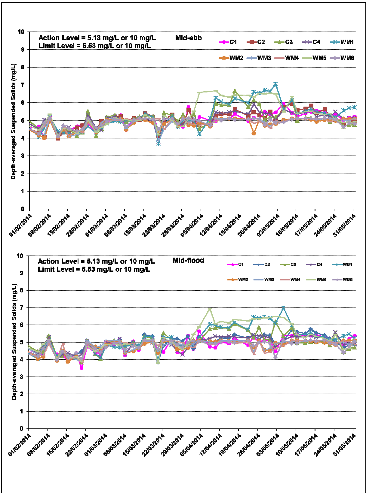
Figure B6 Impact Monitoring – Mean Depth-averaged Level of Suspended Solids (mg/L) between 1 February 2014 and 31 May 2014 at Monitoring Stations for Marine Works.
