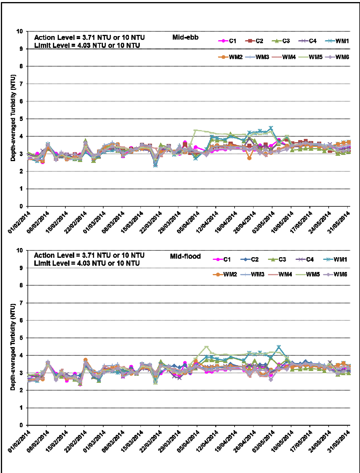
Figure B7 Impact Monitoring – Mean Depth-averaged Level of Turbidity (NTU) between 1 February 2014 and 31 May 2014 at Monitoring Stations for Marine Works.
