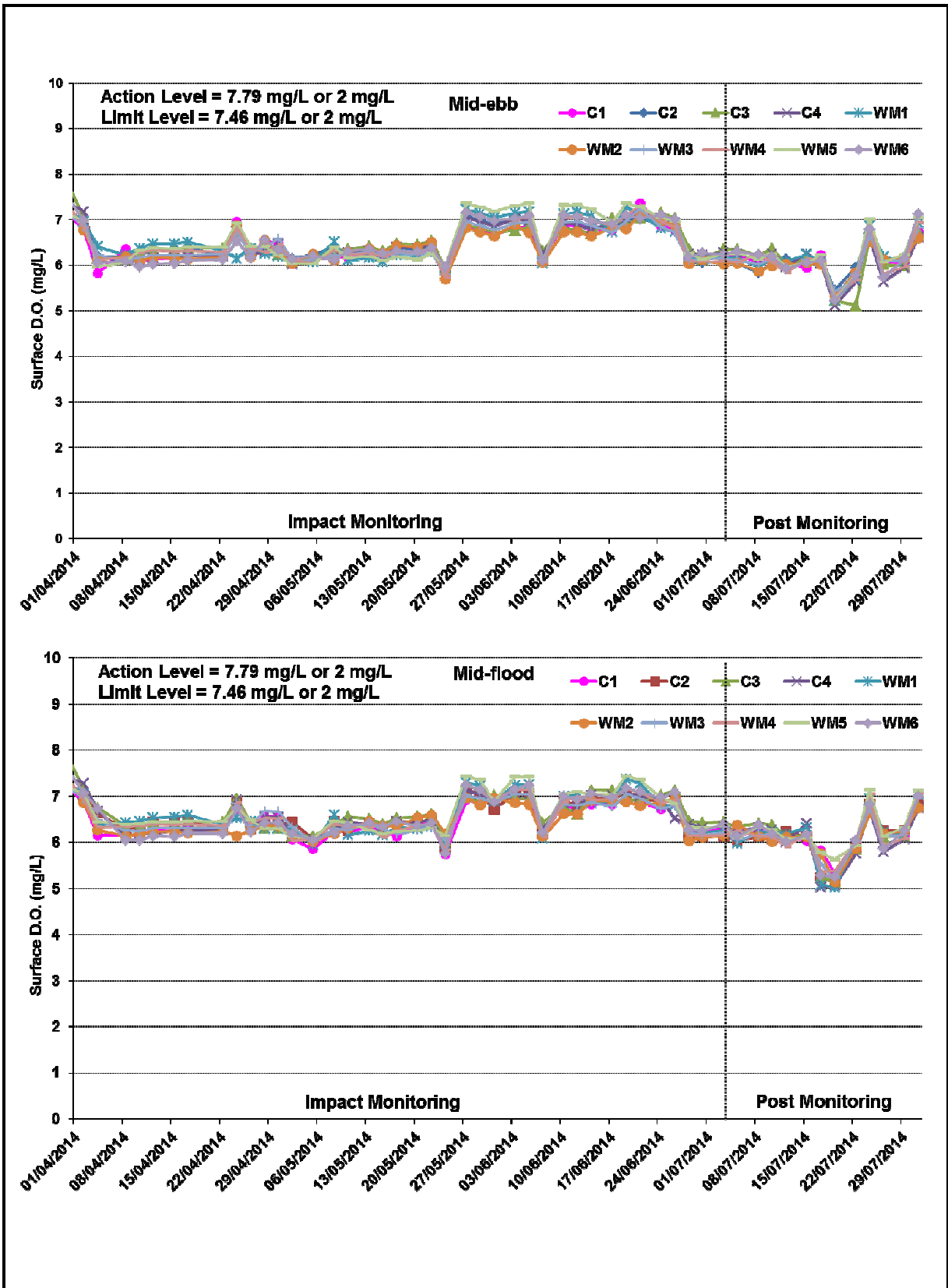
Figure B4 Impact and Post Monitoring – Mean Level of Dissolved Oxygen (mg/L) in surface waters between 1 April 2014 and 31 July 2014 at Monitoring Stations for Marine Works.
