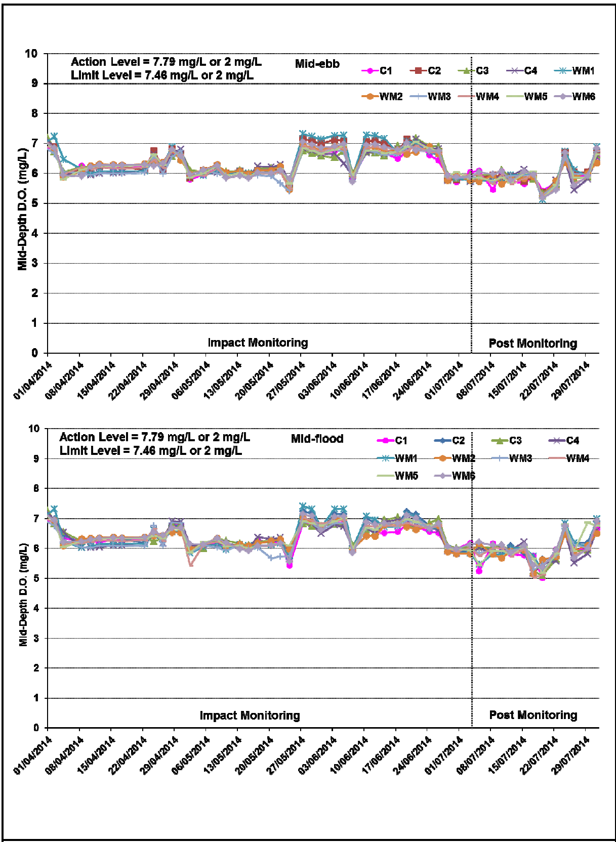
Figure B5 Impact and Post Monitoring – Mean Level of Dissolved Oxygen (mg/L) in mid-depth waters between 1 April 2014 and 31 July 2014 at Monitoring Stations for Marine Works.
