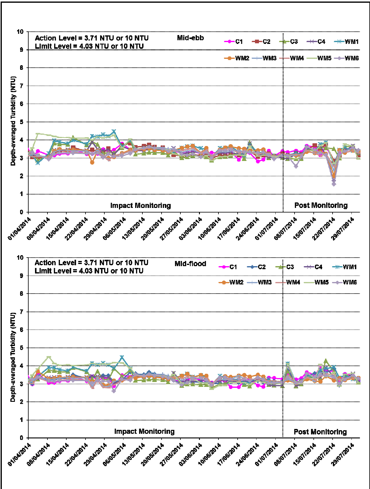
Figure B8 Impact and Post Monitoring – Mean Depth-averaged Level of Turbidity (NTU) between 1 April 2014 and 31 July 2014 at Monitoring Stations for Marine Works.
