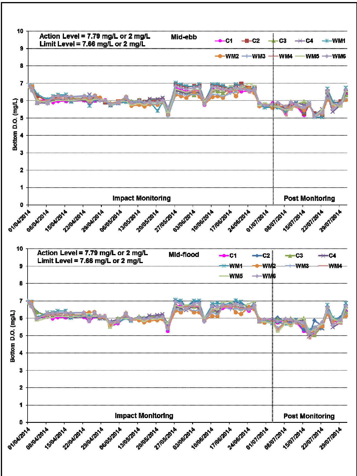
Figure B6 Impact and Post Monitoring – Mean Level of Dissolved Oxygen (mg/L) in bottom waters between 1 April 2014 and 31 July 2014 at Monitoring Stations for Marine Works.
