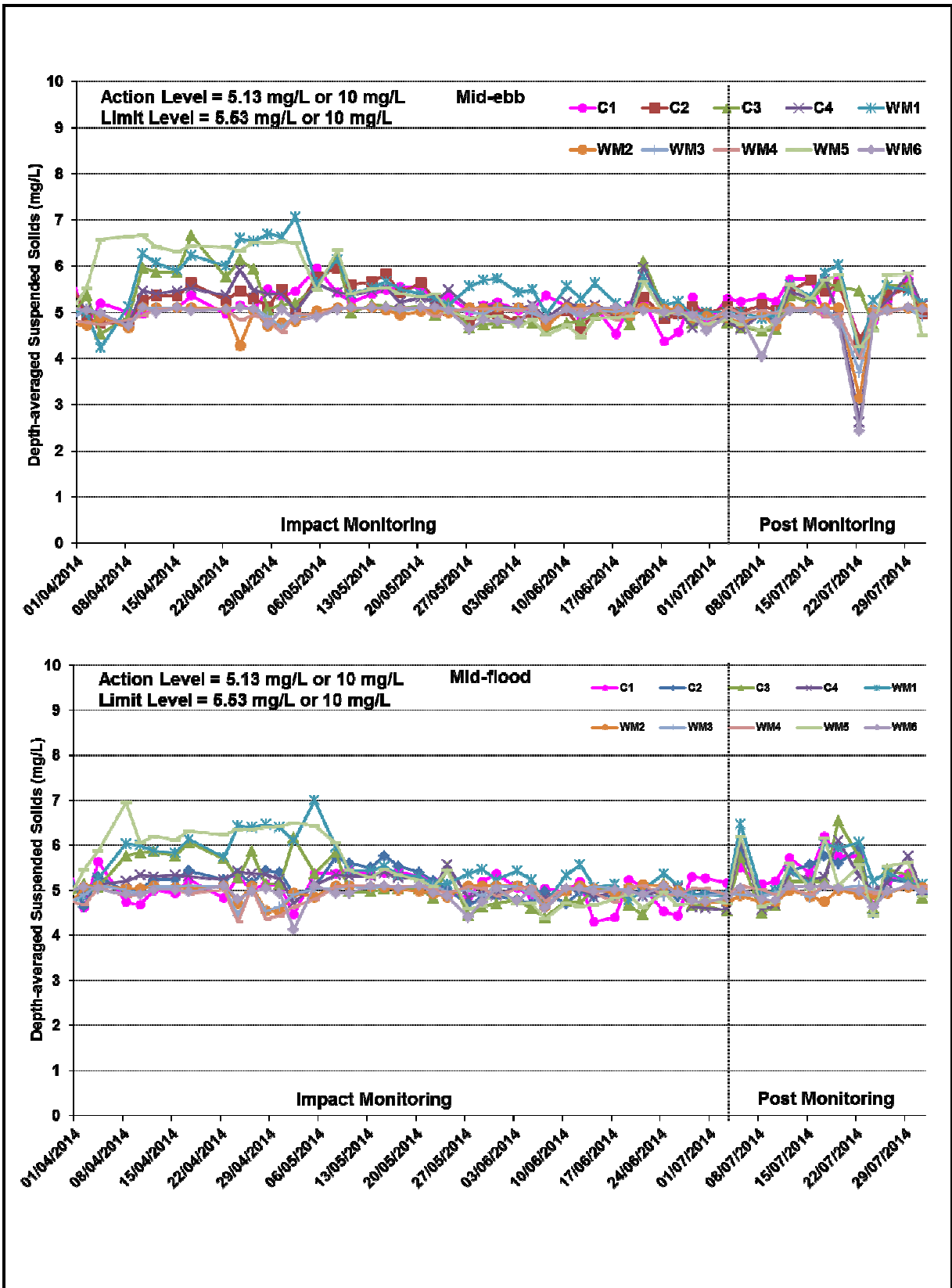
Figure B7 Impact and Post Monitoring – Mean Depth-averaged Level of Suspended Solids (mg/L) between 1 April 2014 and 31 July 2014 at Monitoring Stations for Marine Works.
