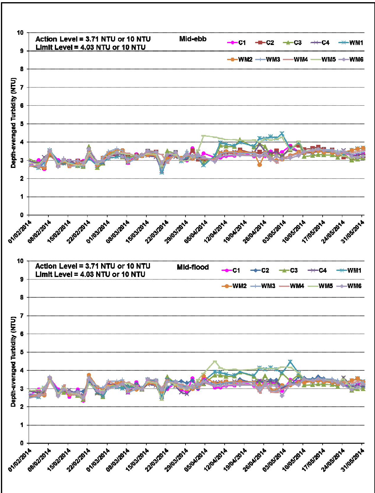
Figure D6 Impact Monitoring – Mean Depth-averaged Level of Turbidity (NTU) between 1 February 2014 and 31 May 2014 at Monitoring Stations for Marine Works.
