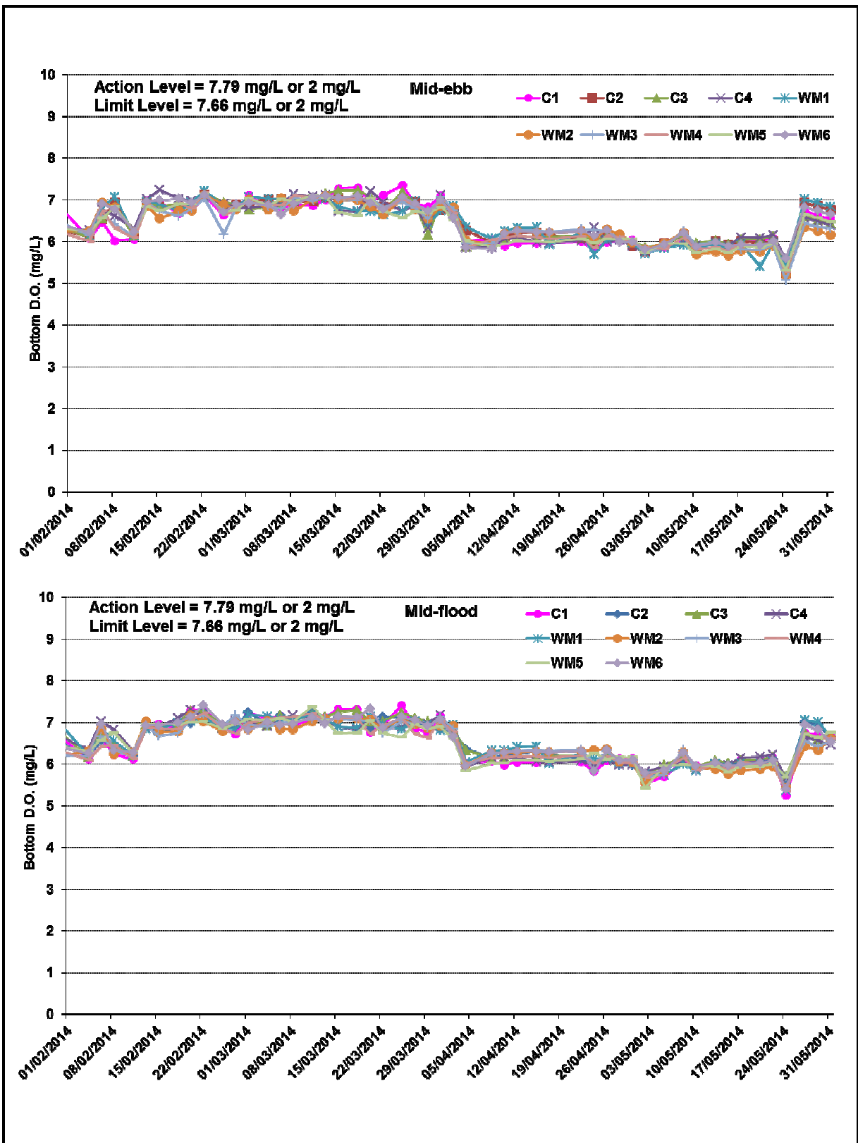
Figure D4 Impact Monitoring – Mean Level of Dissolved Oxygen (mg/L) in bottom waters between 1 February 2014 and 31 May 2014 at Monitoring Stations for Marine Works.
