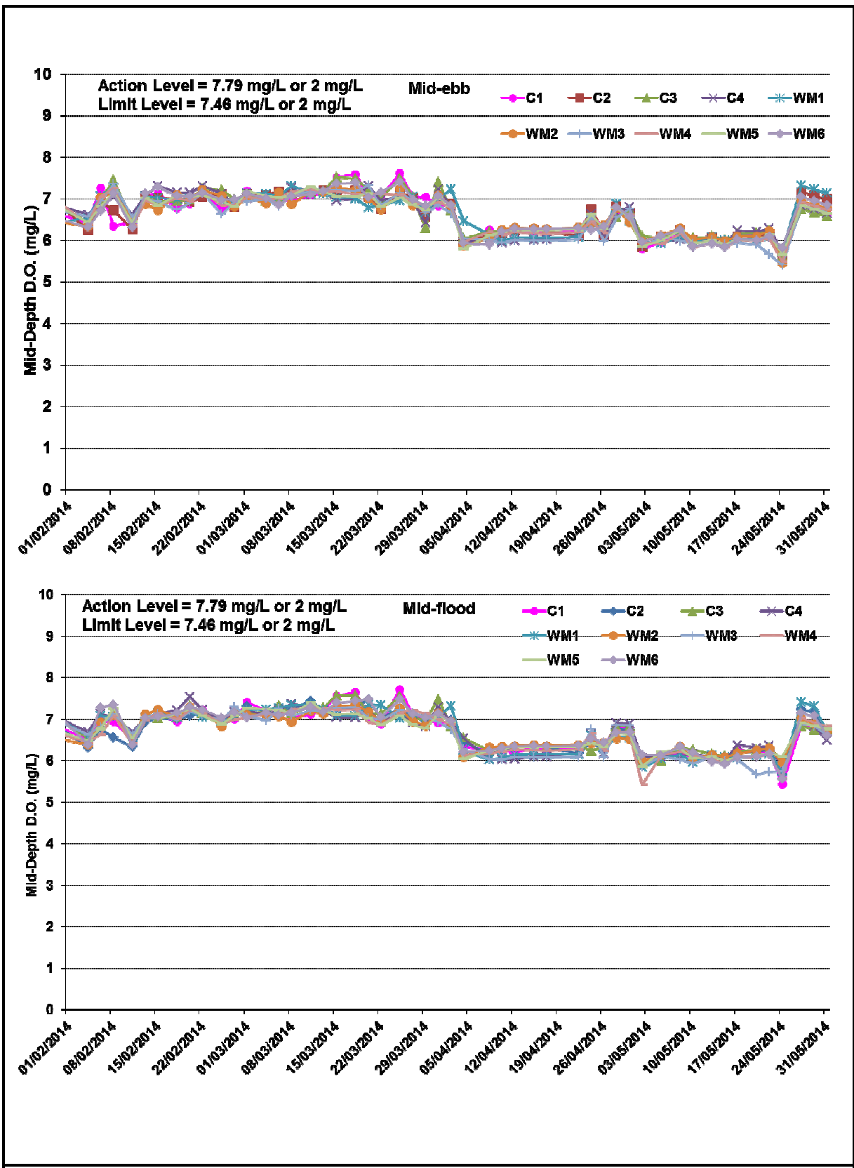
Figure D3 Impact Monitoring – Mean Level of Dissolved Oxygen (mg/L) in mid-depth waters between 1 February 2014 and 31 May 2014 at Monitoring Stations for Marine Works.
