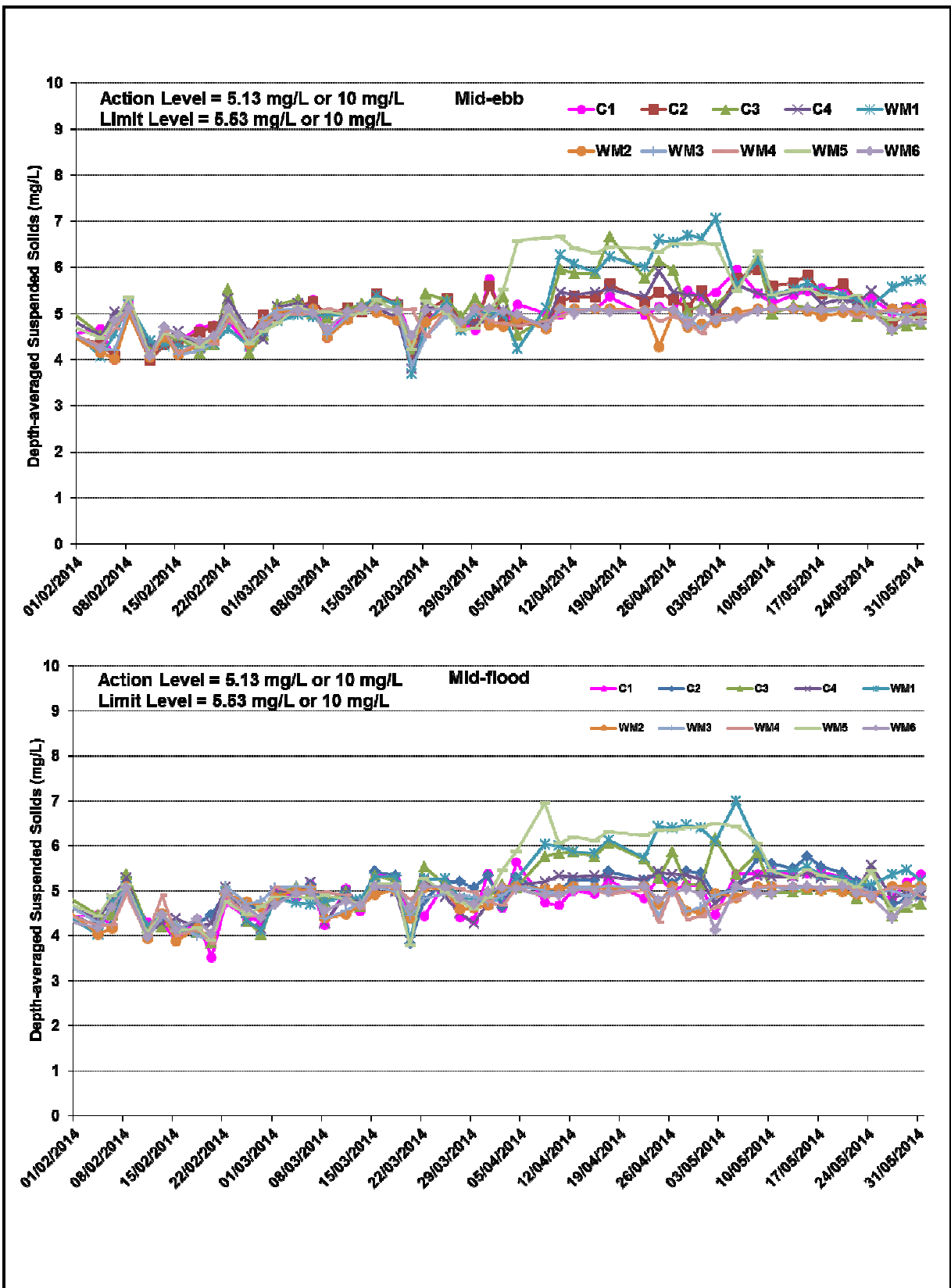
Figure D5 Impact Monitoring – Mean Depth-averaged Level of Suspended Solids (mg/L) between 1 February 2014 and 31 May 2014 at Monitoring Stations for Marine Works.
