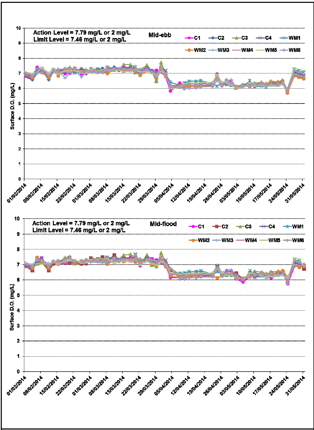
Figure D2 Impact Monitoring – Mean Level of Dissolved Oxygen (mg/L) in surface waters between 1 February 2014 and 31 May 2014 at Monitoring Stations for Marine Works.
