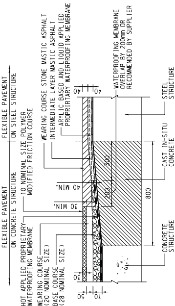
TYPICAL DETAILS FOR FLEXIBLE PAVEMENT ON CONCRETE STRUCTURE
