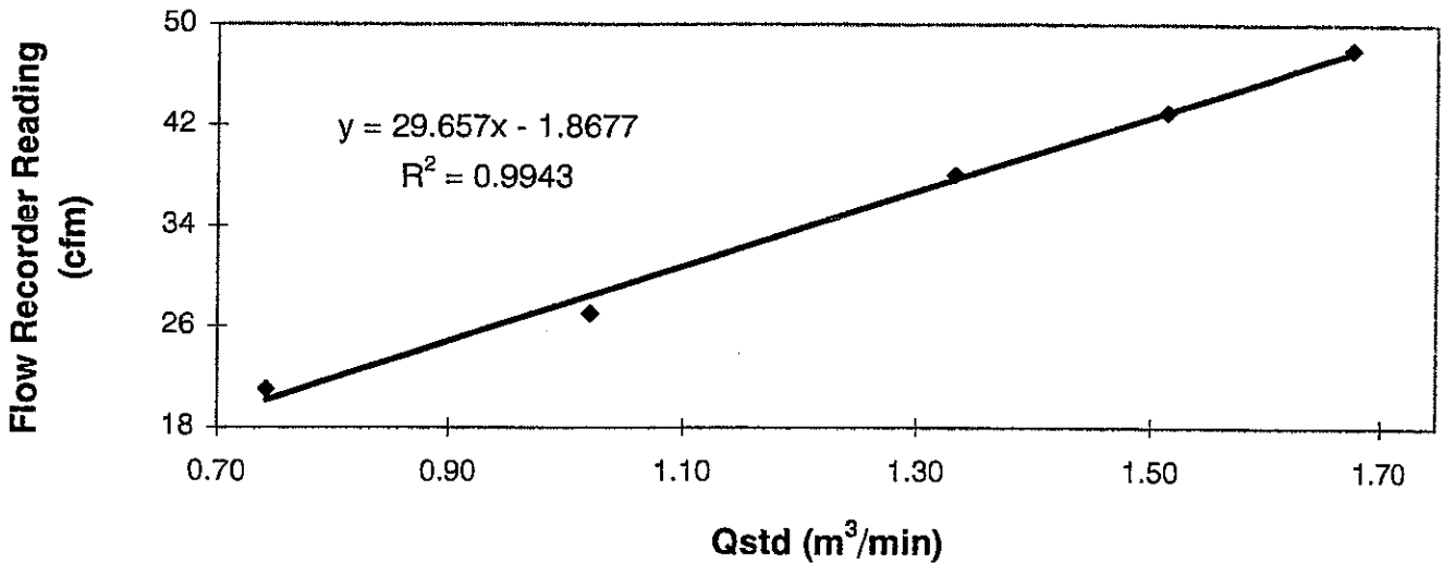
Air Sampler 1176 Calibration Curve Site: Tseung Kwan O (AA2) Date of Calibration: 20 September 2006
