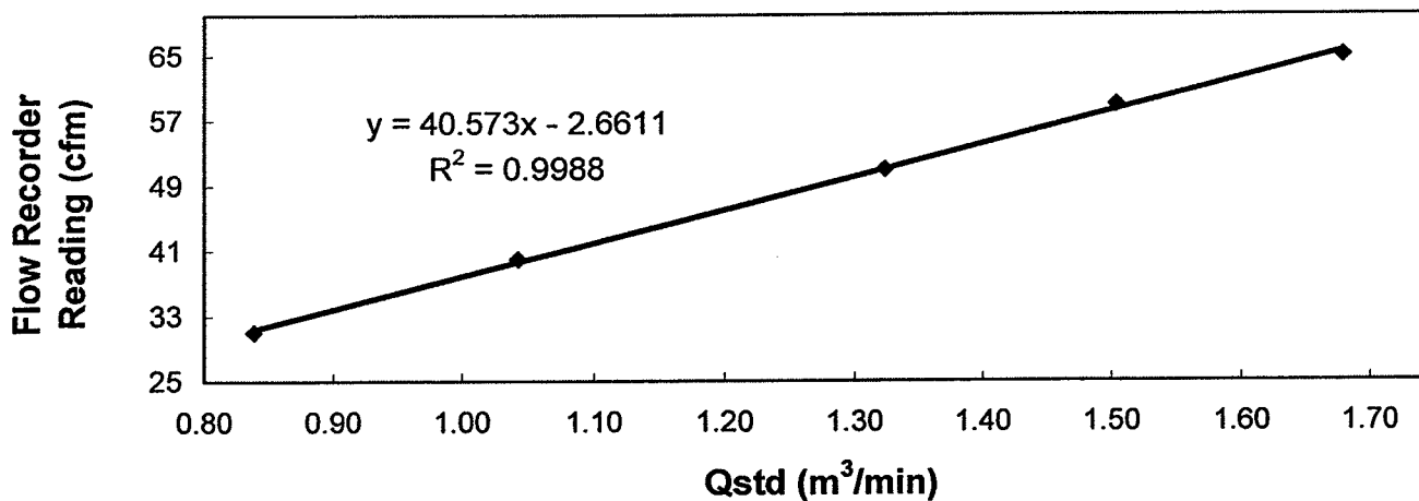
Sampler 1176 Calibration Curve Site: Tseung Kwan O (A-2) Date of Calibration: 23 January 2008
