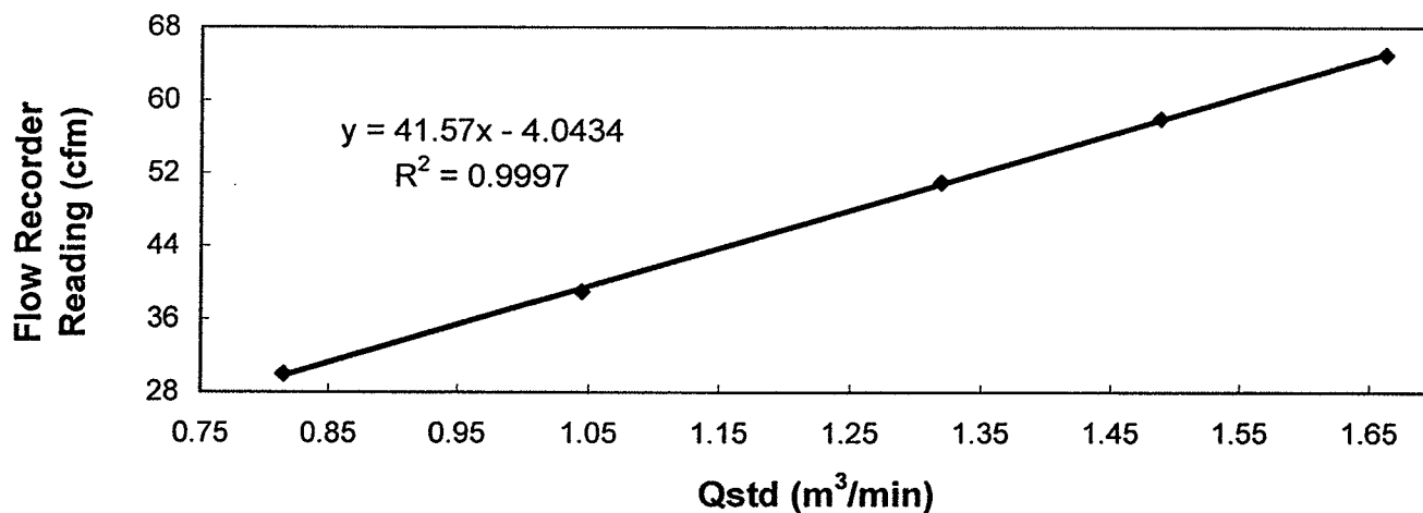
Sampler 10347 Calibration Curve Site: Tseung Kwan O (A-1) Date of Calibration: 23 November 2007
