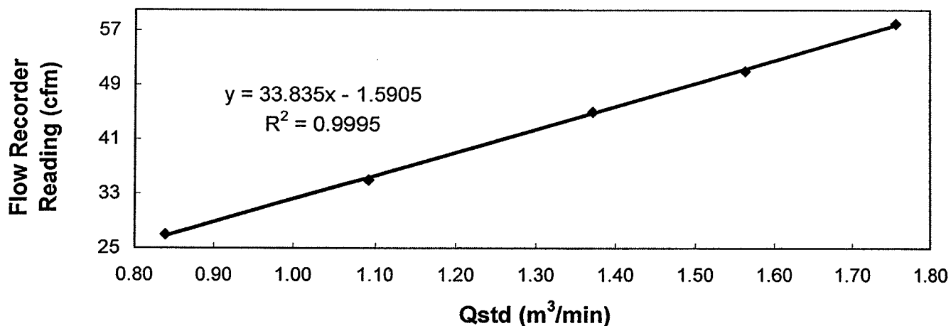
Sampler 10347 Calibration Curve Site: Tseung Kwan O (A-1) Date of Calibration: 23 January 2008
