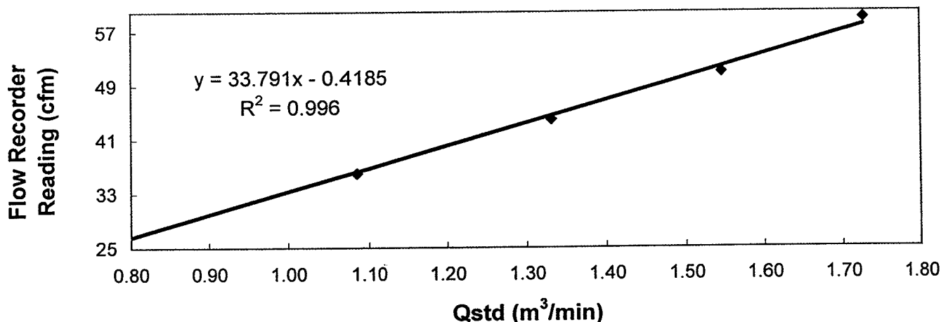
Sampler 10347 Calibration Curve Site: Tseung Kwan O (A-1) Date of Calibration: 23 May 2008
