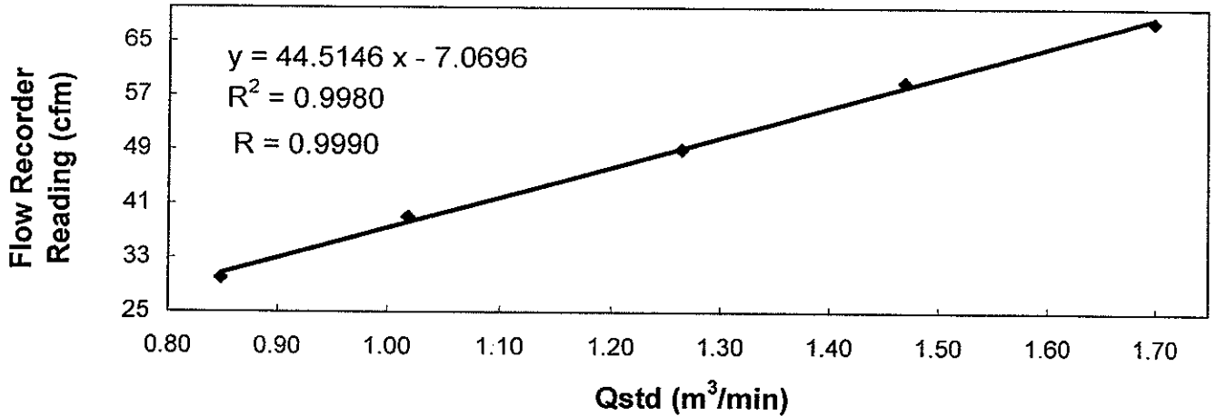
Sampler 1176 Calibration Curve Site: Tseung Kwan O (A-2) Date of Calibration: 23 July 2008
