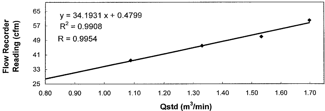
Sampler 10347 Calibration Curve Site: Tseung Kwan O (A-1) Date of Calibration: 23 July 2008
