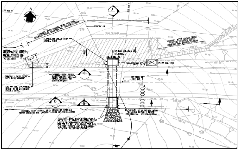
LAYOUT PLAN SCALE 1 : 200
