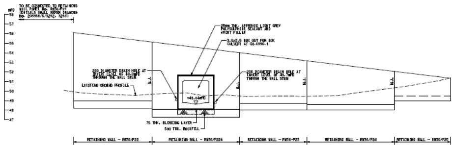
ELEVATION B - B (DEVELOPED) SCALE 1 : 100
