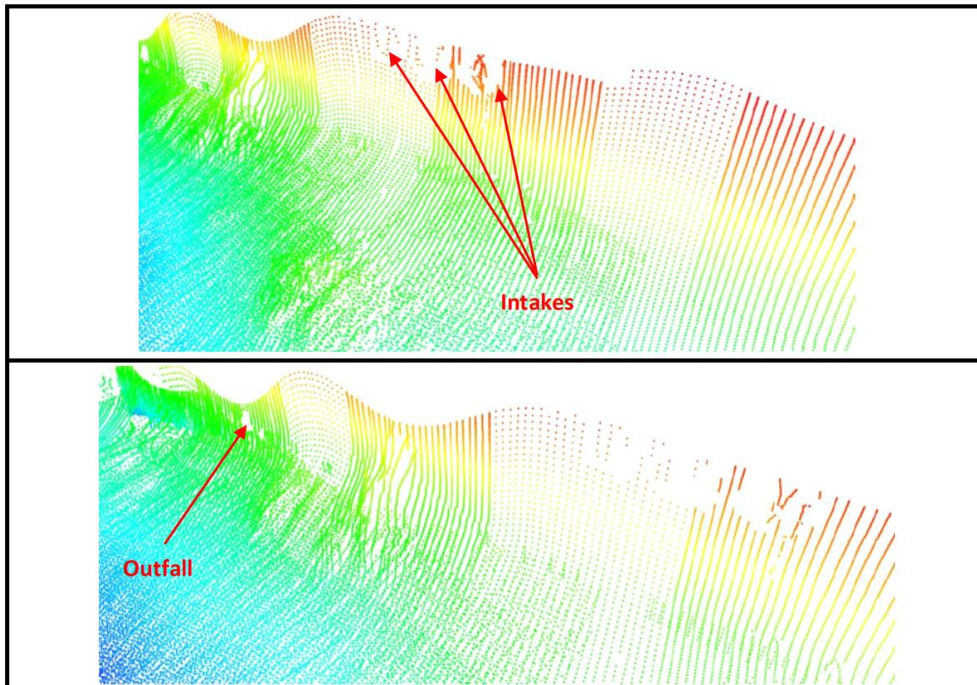
Figure 6: 3D perspective view of raw MBES soundings at intakes and outfall location
