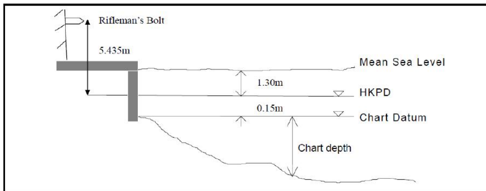
Figure 2: Definitions of Vertical Datum in Hong Kong (SMO, Lands Department HKSAR, 2018)
