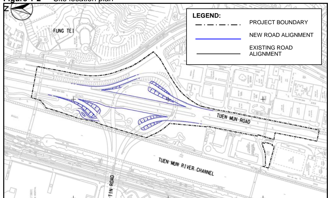
Figure 1-2 Site location plan
