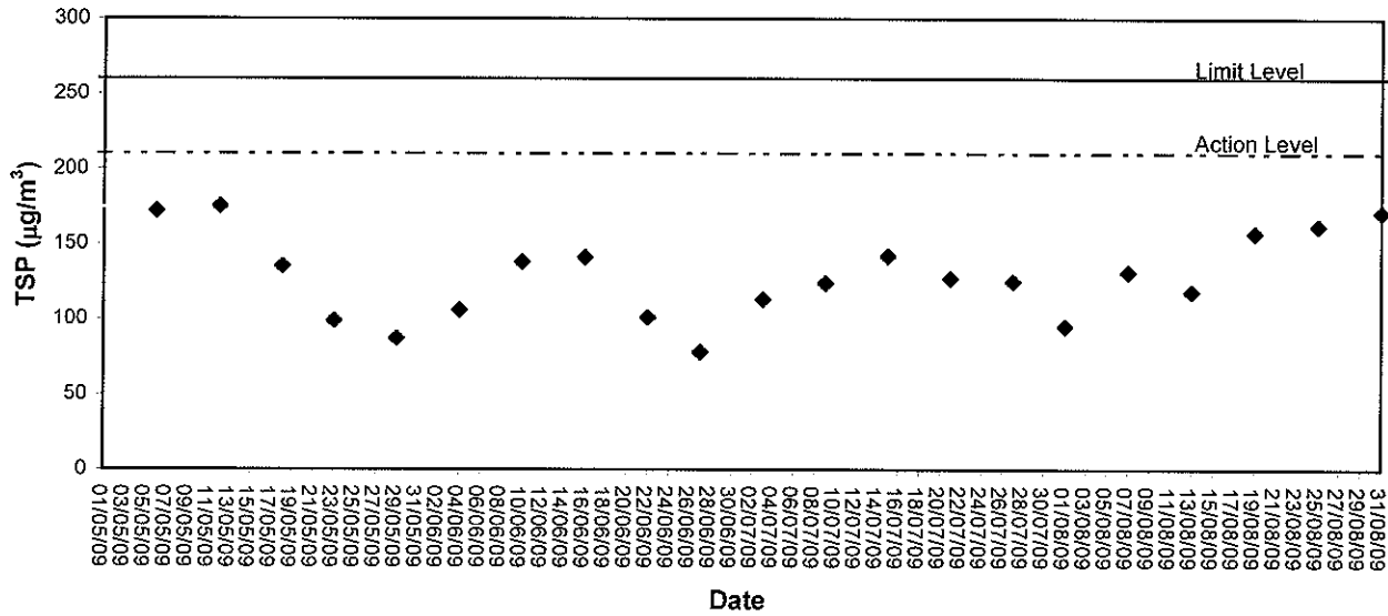
24-hour TSP level at TKO-A2 (Site Egress)
