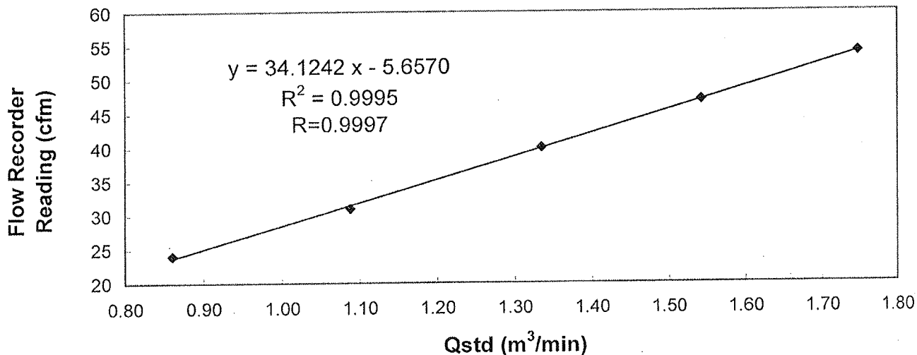
Sampler 2485 Calibration Curve Site: Sorting TKO (TKO2)
