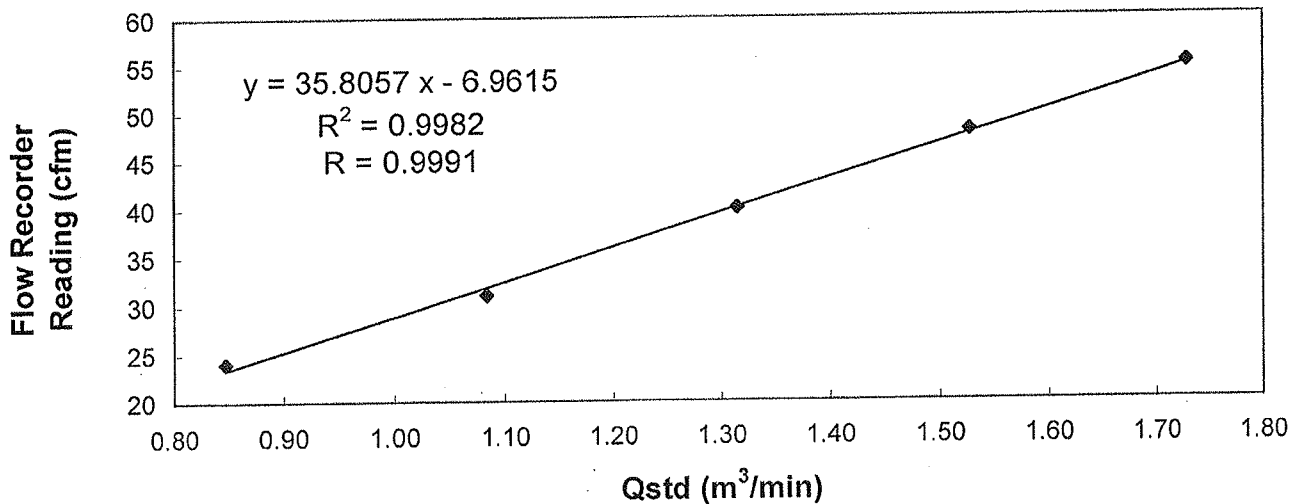
Sampler 2485 Calibration Curve Site: TKO CWSF - TKO2
