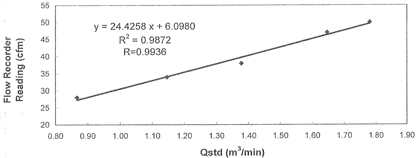
Sampler 1172 Calibration Curve Site: Tseung Kwan O 137 (TKO-A2a)
