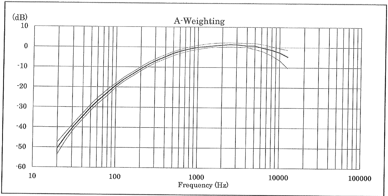
Relative free field frequency response
