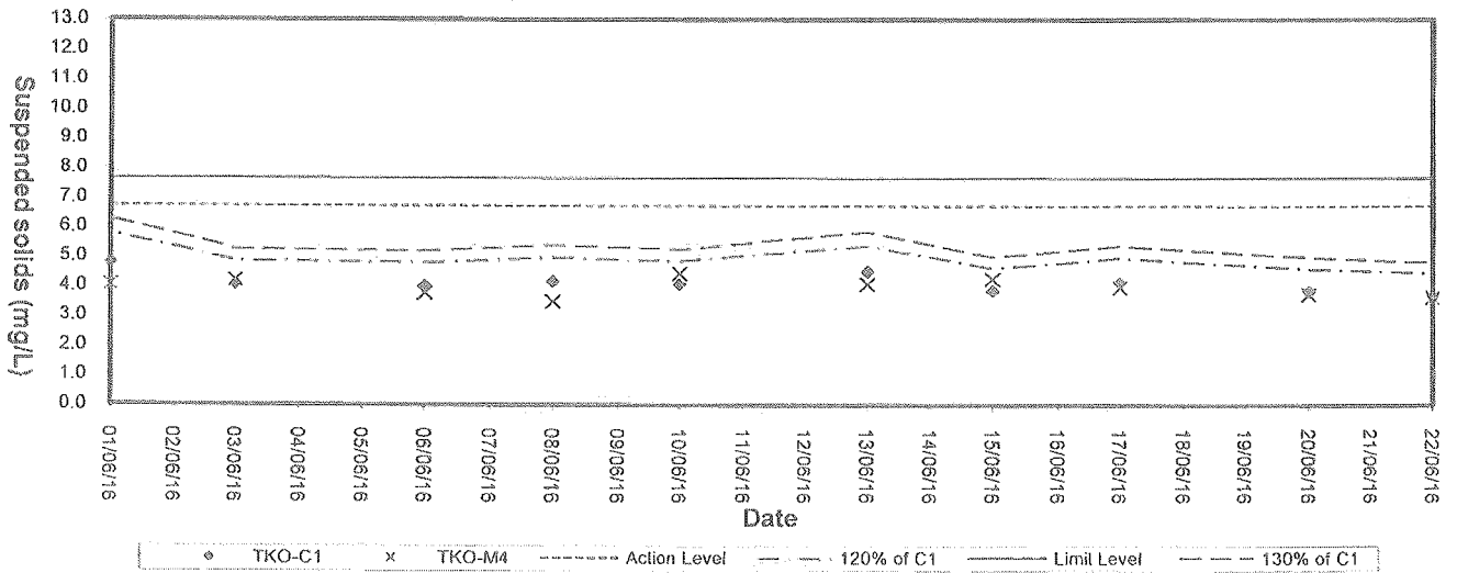
Suspended Solids (Depth-average) at Mid-Ebb Tide
