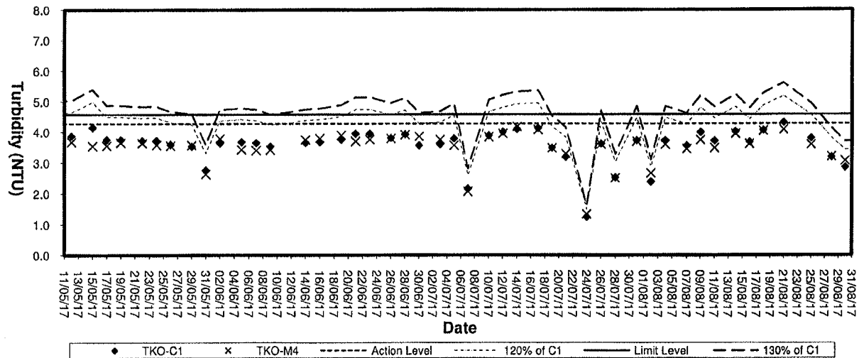
Turbidity(Depth-average) at Mid-Ebb Tide
