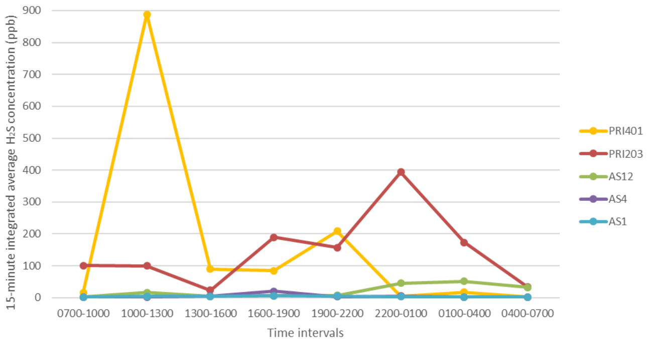
Trend of 15-minute Integrated Average H 2 S Concentrations at Different Monitoring Stations across Different Time Intervals
