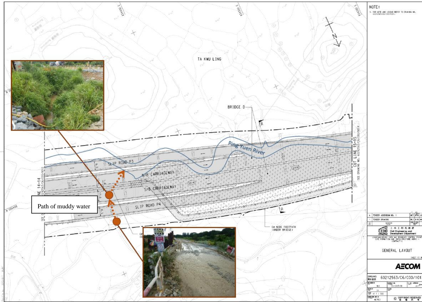
Figure 2: Location of the concerned haul road and channel
