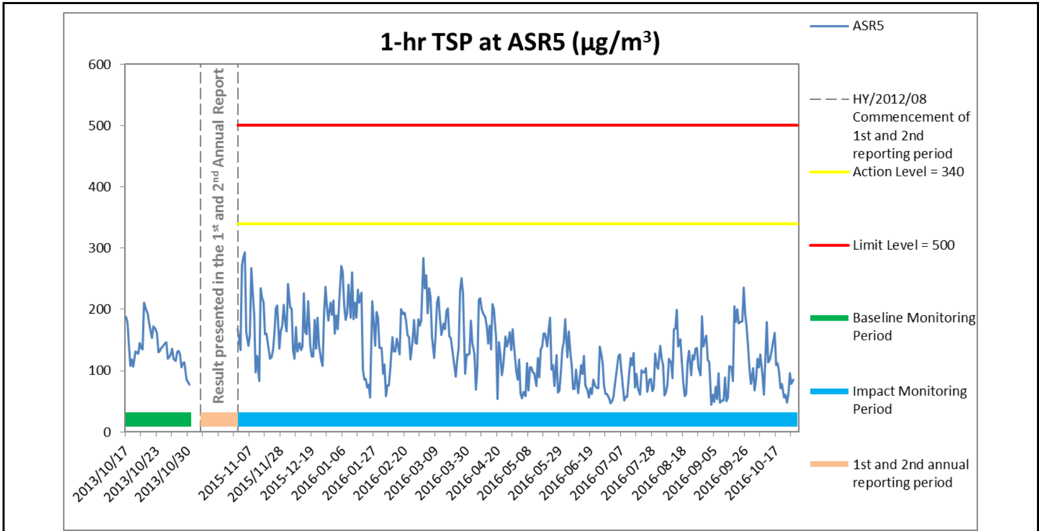
Figure D.4 Baseline & Impact Monitoring - 1-hour Total Suspended Particulates ( \mu\text{g}/\text{m}^3 ) at ASR5 between 17 October 2013 and 31 October 2016 during Baseline & Impact Monitoring period. Weather condition within the reporting period varied between sunny to rainy. The overall monitoring results were not affected by weather conditions. Major land-based construction activities included: Construction of Cross Passage Tympanum, Box Culvert Extension, CSM Ground Treatment, Diaphragm Wall Construction, TBM Tunnel Works & Excavation of sub-sea tunnel. Ref: 0212330_Impact AQM graphs_3rdAnnual_REV a.xlsx
