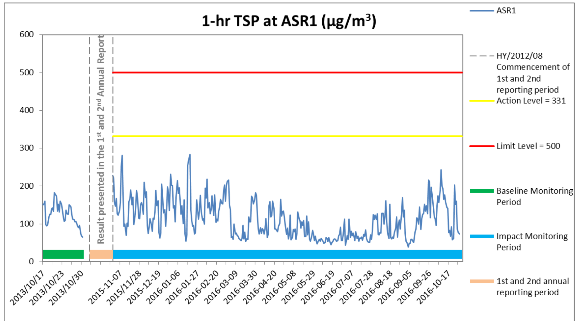
Figure D.3 Baseline & Impact Monitoring - 1-hour Total Suspended Particulates ( \mu\text{g}/\text{m}^3 ) at ASR1 between 17 October 2013 and 31 October 2016 during Baseline & Impact Monitoring period. Weather condition within the reporting period varied between sunny to rainy. The overall monitoring results were not affected by weather conditions. Major land-based construction activities included: Construction of Cross Passage Tympanum, Box Culvert Extension, CSM Ground Treatment, Diaphragm Wall Construction, TBM Tunnel Works & Excavation of sub-sea tunnel. Ref: 0212330_Impact AQM graphs_3rdAnnual_REV a.xlsx
