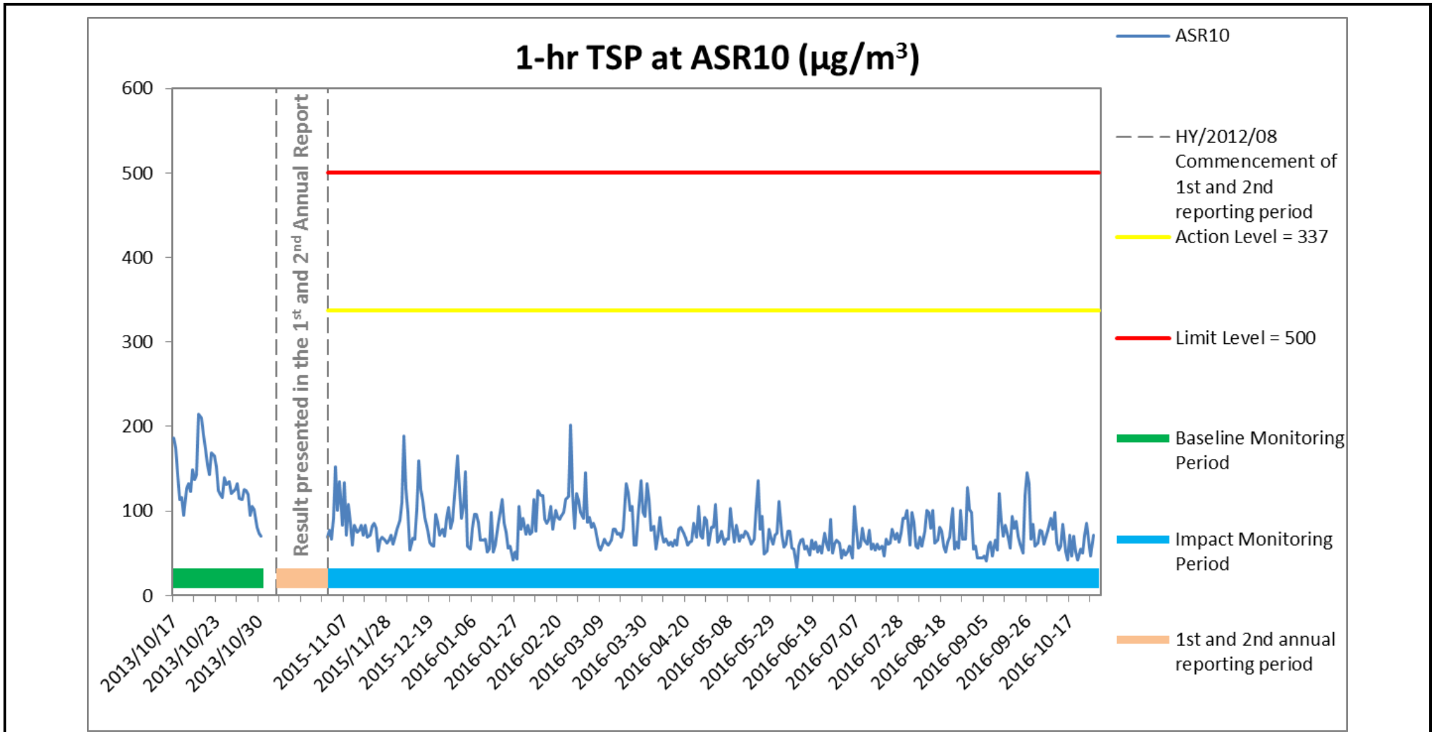
Figure D.5 Baseline & Impact Monitoring - 1-hour Total Suspended Particulates ( \mu\text{g}/\text{m}^3 ) at ASR10 between 17 October 2013 and 31 October 2016 during Baseline & Impact Monitoring period. Weather condition within the reporting period varied between sunny to rainy. The overall monitoring results were not affected by weather conditions. Major land-based construction activities included: Construction of Cross Passage Tympanum, Box Culvert Extension, CSM Ground Treatment, Diaphragm Wall Construction, TBM Tunnel Works & Excavation of sub-sea tunnel. Ref: 0212330_Impact AQM graphs_3rdAnnual_REV a.xlsx
