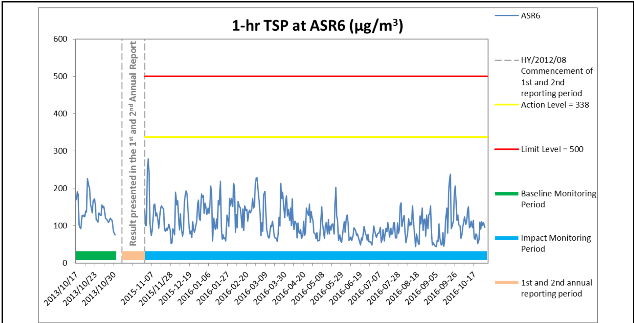
Figure D.2 Baseline & Impact Monitoring - 1-hour Total Suspended Particulates ( \mu\text{g}/\text{m}^3 ) at AQMS2/ASR6 between 17 October 2013 and 31 October 2016 during Baseline & Impact Monitoring period. Weather condition within the reporting period varied between sunny to rainy. The overall monitoring results were not affected by weather conditions. Major land-based construction activities included: Construction of Cross Passage Tympanum, Box Culvert Extension, CSM Ground Treatment, Diaphragm Wall Construction, TBM Tunnel Works & Excavation of sub-sea tunnel. Ref: 0212330_Impact AQM graphs_3rdAnnual_REV a.xlsx
