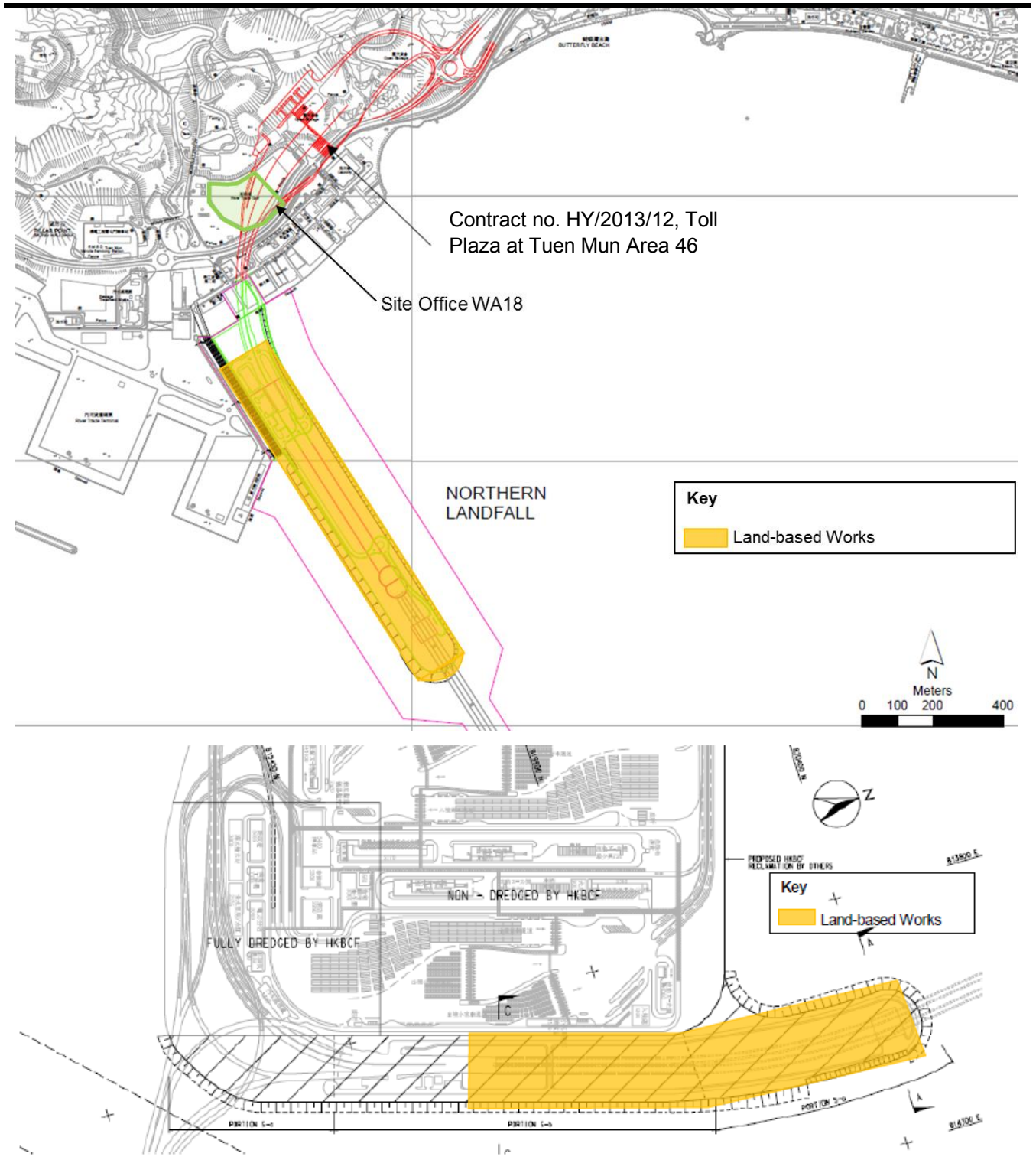
Figure 1.2 Locations of Construction Activities – November 2015 to October 2016
