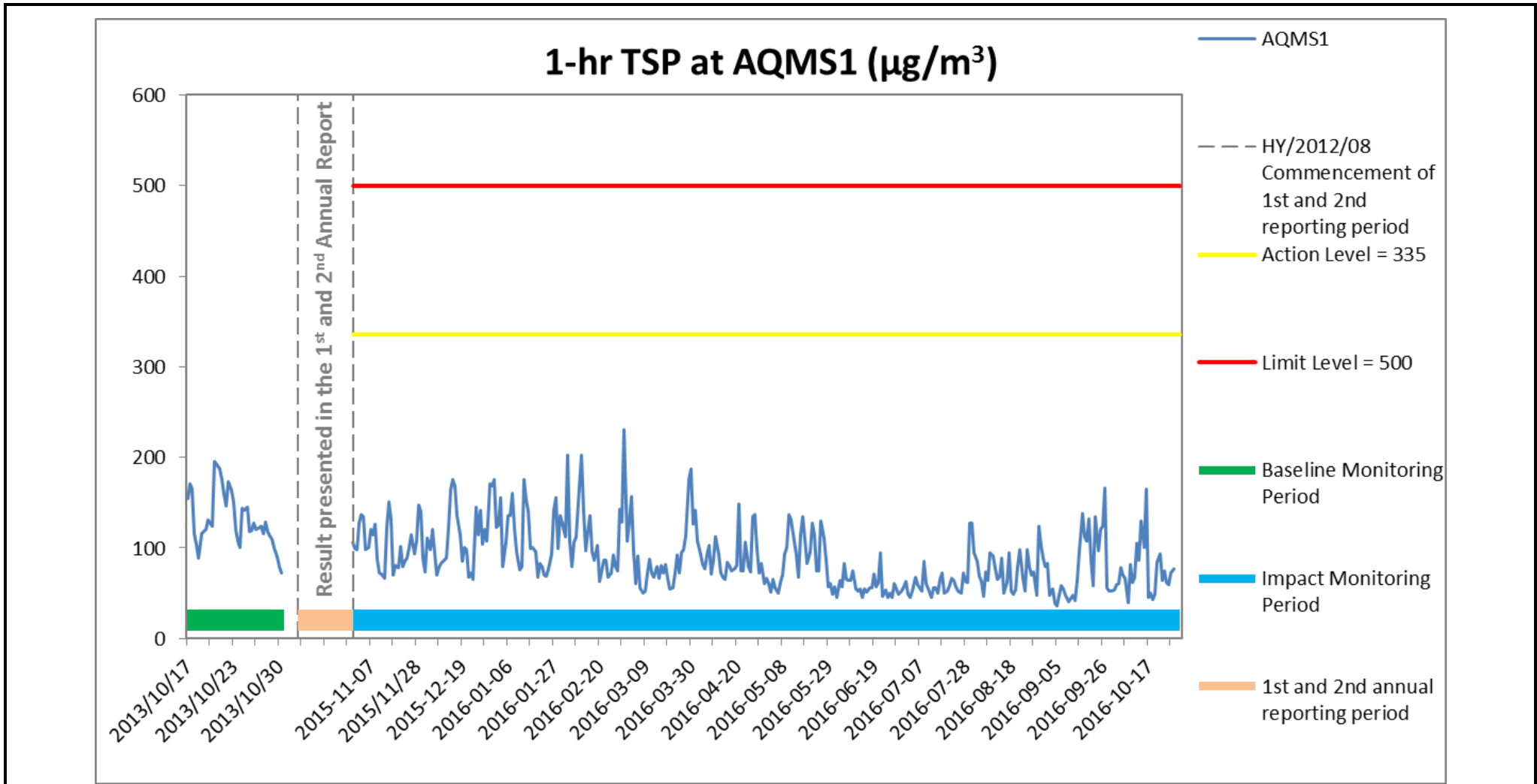
Figure D.1 Baseline & Impact Monitoring - 1-hour Total Suspended Particulates ( \mu\text{g}/\text{m}^3 ) at AQMS1 between 17 October 2013 and 31 October 2016 during Baseline & Impact Monitoring period. Weather condition within the reporting period varied between sunny to rainy. The overall monitoring results were not affected by weather conditions. Major land-based construction activities included: Construction of Cross Passage Tympanum, Box Culvert Extension, CSM Ground Treatment, Diaphragm Wall Construction, TBM Tunnel Works & Excavation of sub-sea tunnel. Ref: 0212330_Impact AQM graphs_3rdAnnual_REV a.xlsx
