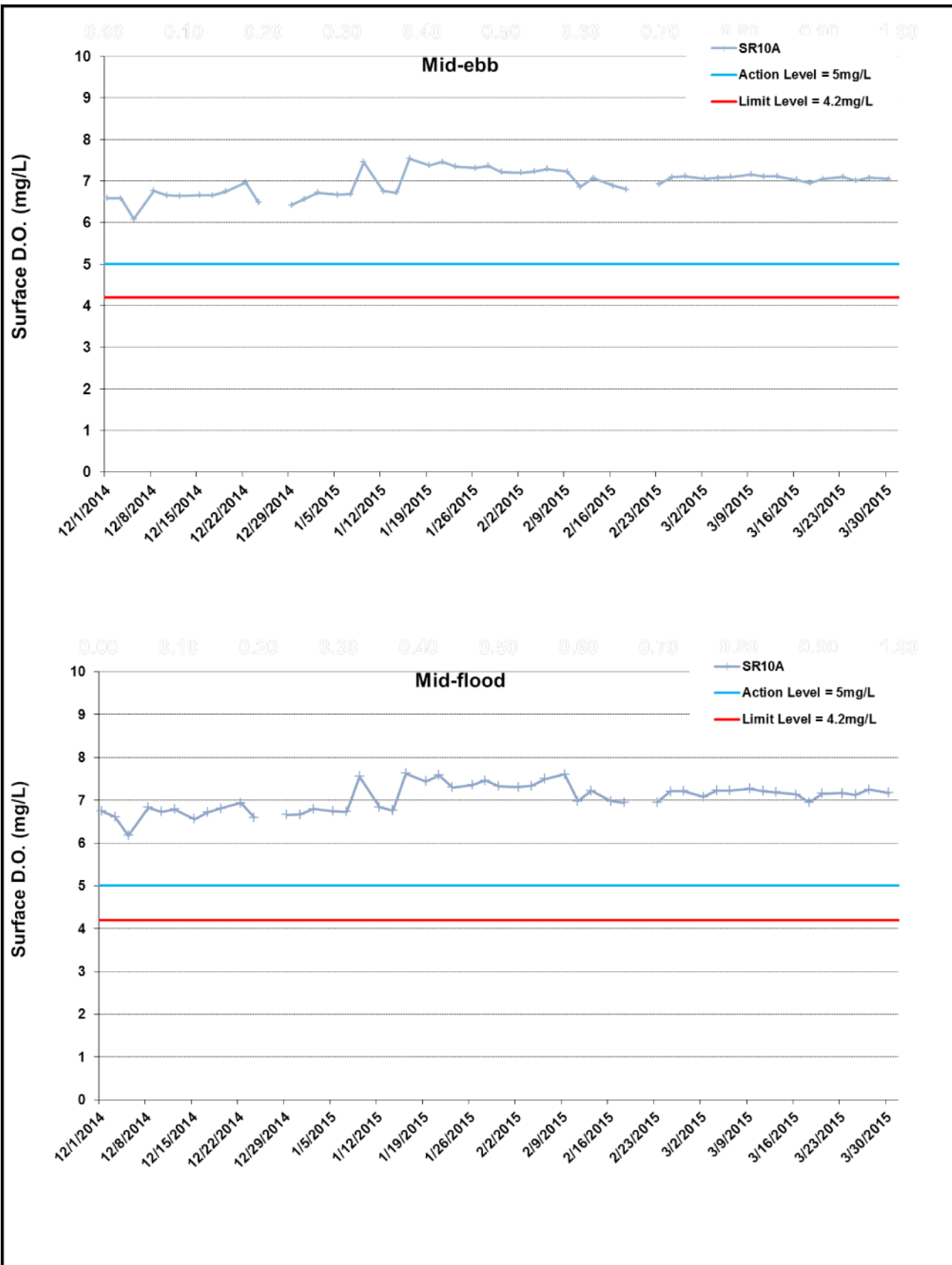
Figure I7 Impact Monitoring - Mean Level of Dissolved Oxygen (mg/L) in surface waters between 1 December 2014 and 31 March 2015 at SR10A. The weather conditions during the monitoring period varied mostly from sunny to cloudy. Only minor marine works included rock bund deposition for marine sheet pile remedial works was carried out from 1 January 2015 to 28 February 2015. WQM on 20 February 2015 was postponed to 23 February 2015.
