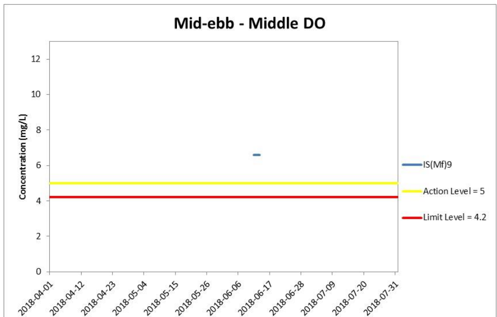
Figure J10 Impact Monitoring – Mean Level of Dissolved Oxygen (mg/L) in mid-depth waters during mid-ebb tide between 1 April and 31 July 2018 at IS(Mf)16 and IS(Mf)9.
