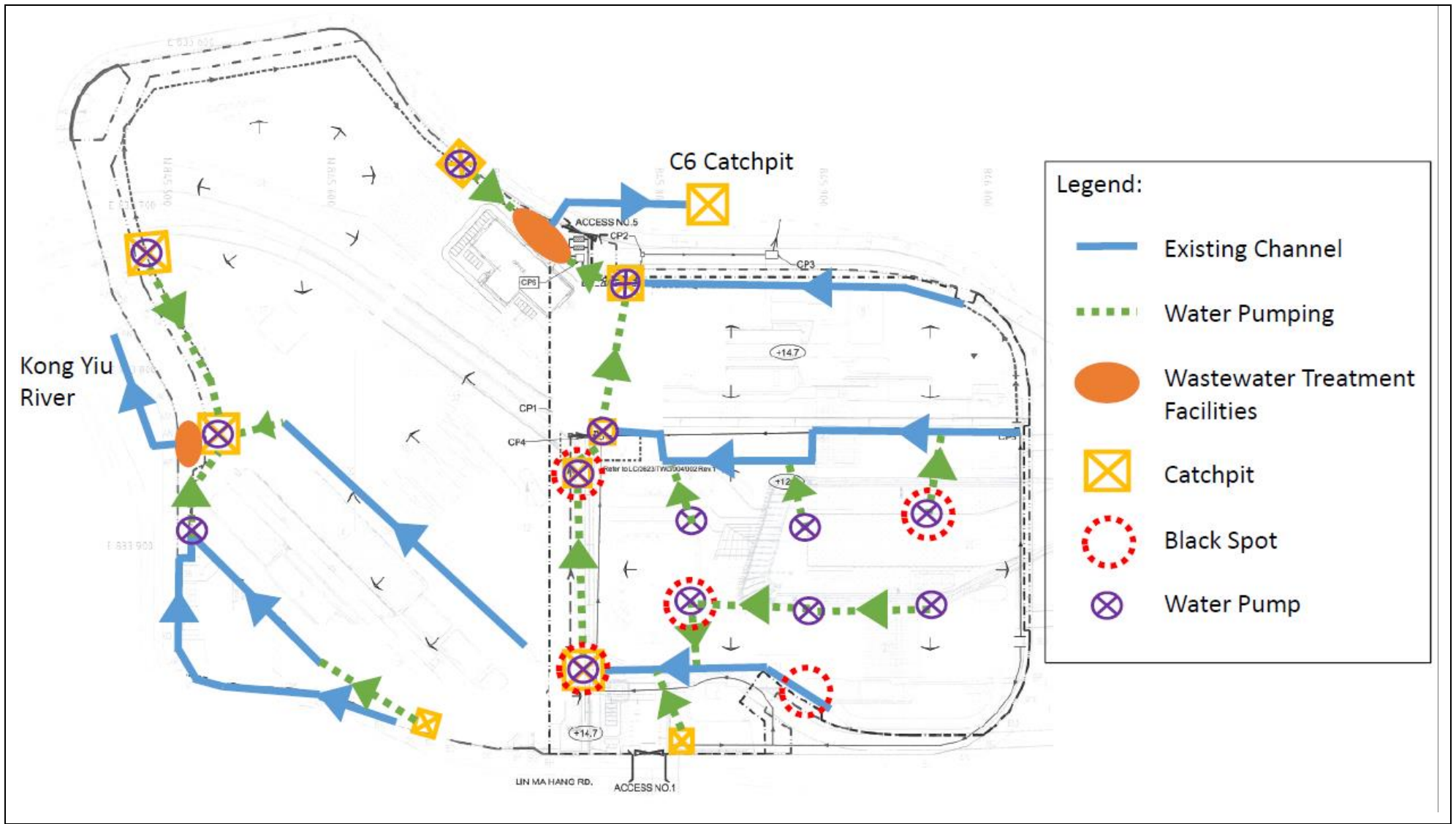
Figure 3 Drainage Plan
