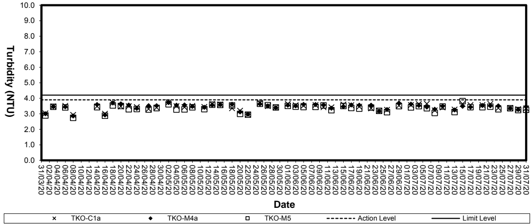
Turbidity (Depth-average) at Mid-Flood Tide (3RS project)
