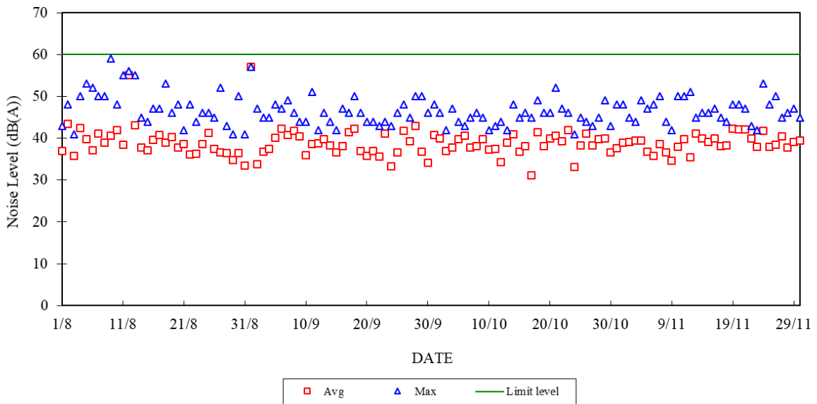
Construction Noise Monitoring in August - November 2023 NSR at School within Tai Wan San Tsuen 07:00-23:00 hrs on Holidays and 19:00-23:00 hrs on All Other Days
