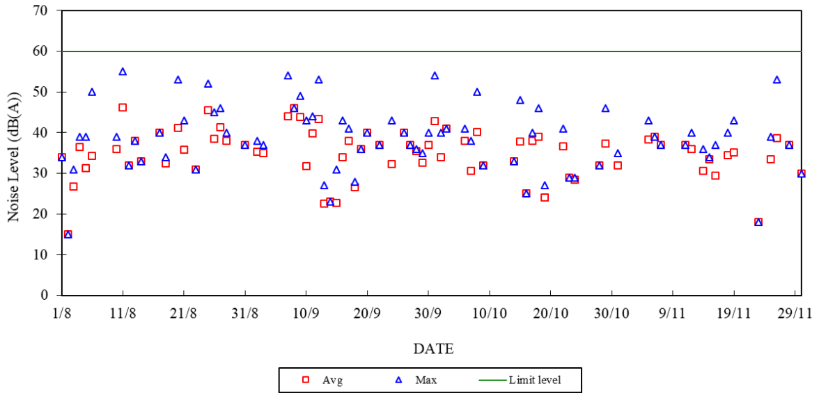
Construction Noise Monitoring in August - November 2023 NSR at Long Tsai Tsuen/Hung Shing Ye 07:00-23:00 hrs on Holidays and 19:00-23:00 hrs on All Other Days
