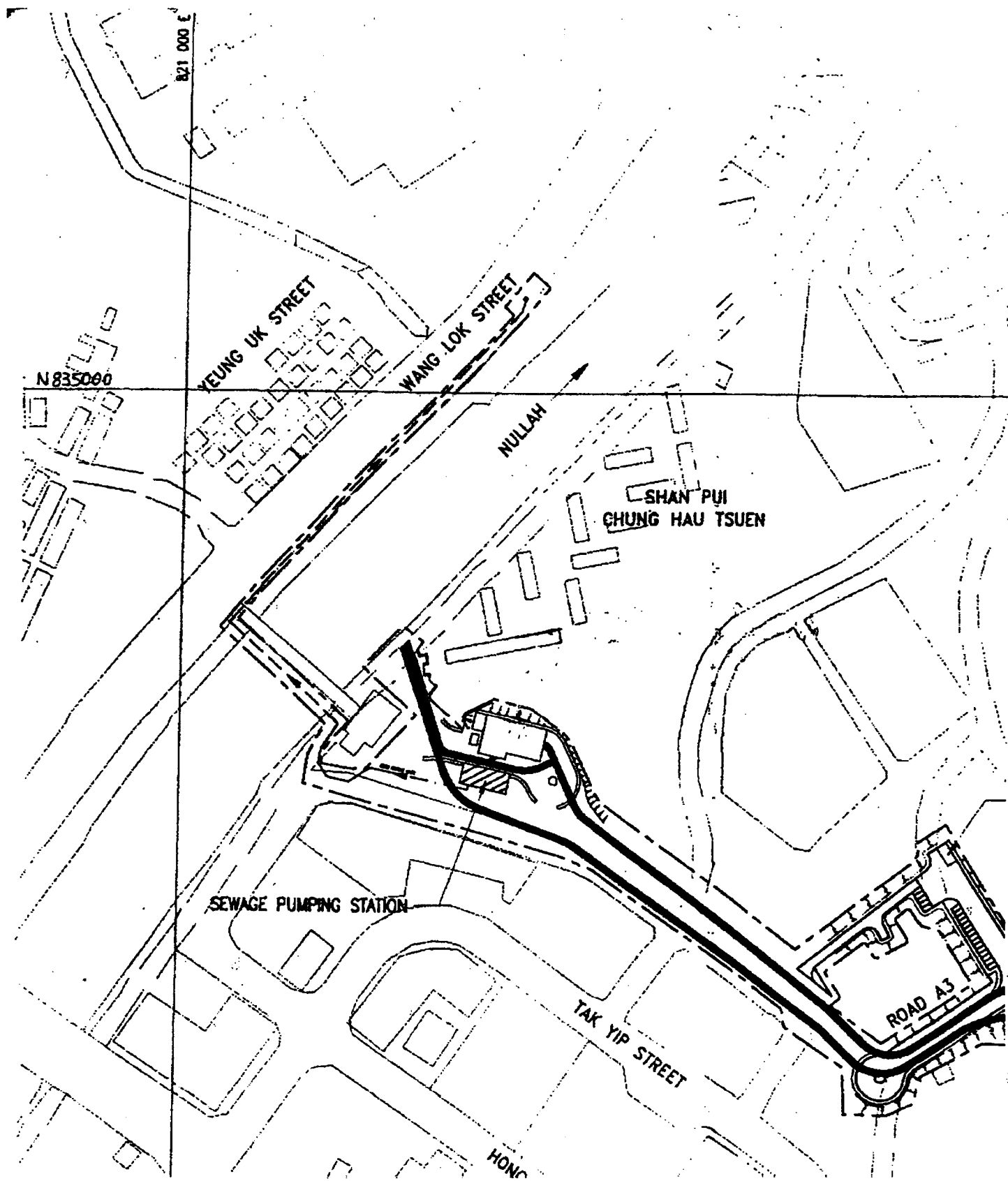
Drawing 1 - Location of Sewage Pumping Station at Tung Tau Industrial Area, Yuen Long
