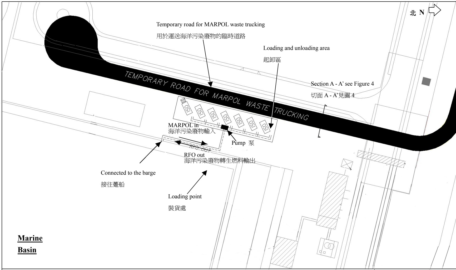
SCHEMATIC SITE LAYOUT OF TEMPORARY MARPOL WASTE RECEPTION FACILITY
