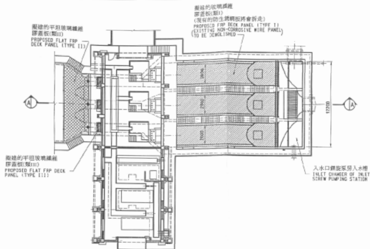
螺旋泵房上蓋 - 平面圖 COVER FOR INLET PUMPING STATION - PLAN
