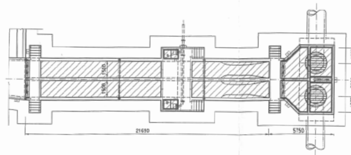
水槽上蓋 - 平面圖 COVER FOR FLUME CHANNELS - PLAN
