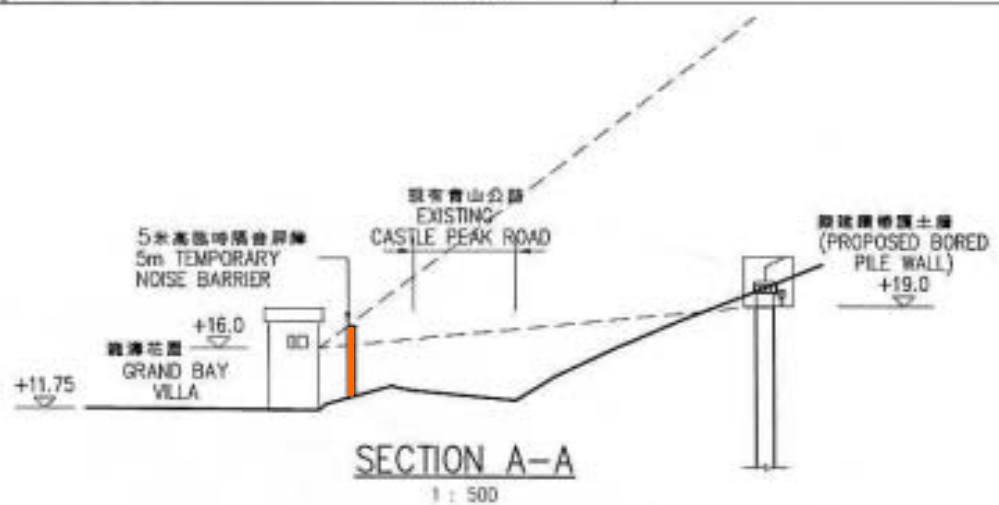
Castle Peak Road Improvement Between Area 2 and Ka Loon Tsuen, Tsuen Wan Proposed Temporary Noise Barriers at Grand Bay Villa
