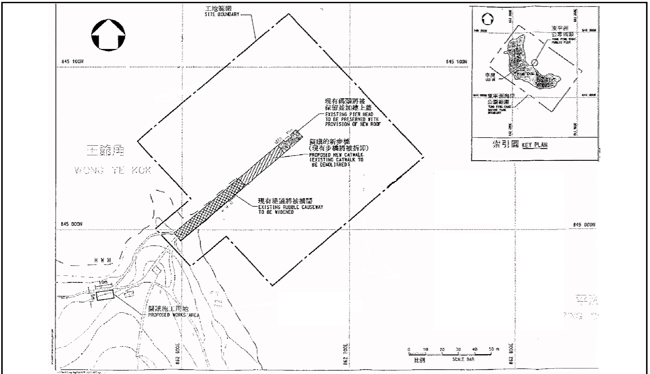
Figure 1: Improvement Works to Tung Ping Chau Public Pier – Location Plan
