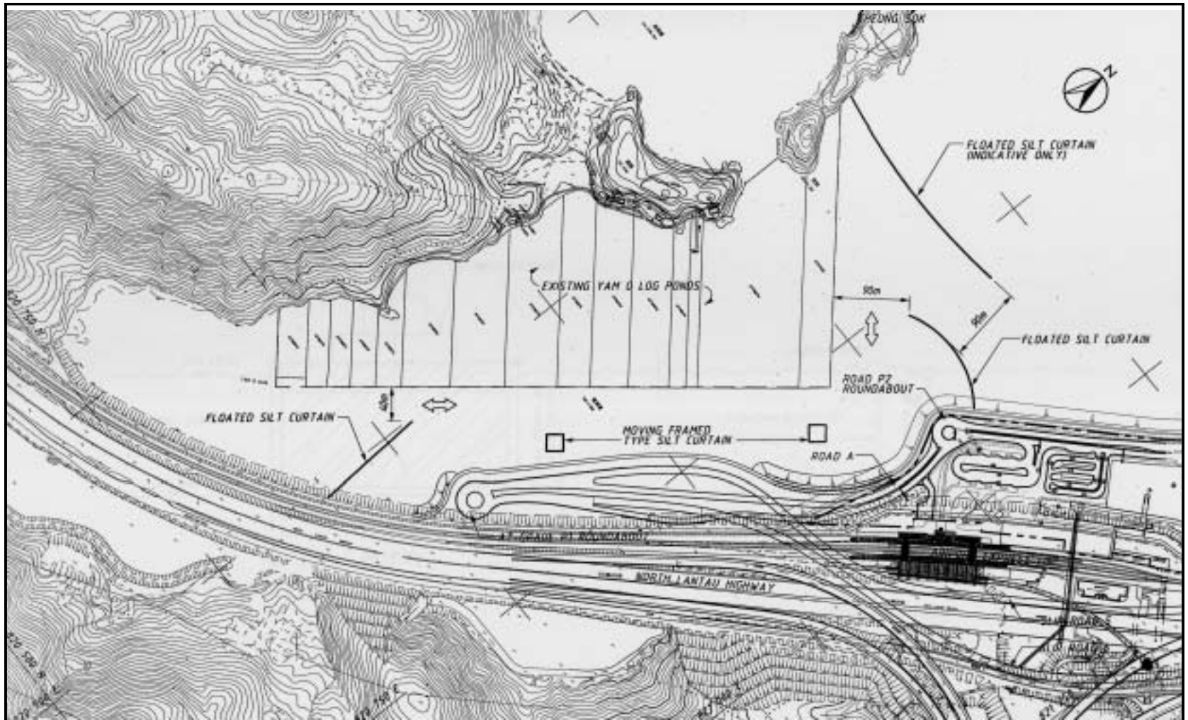
Figure 2 – Silt Curtain Arrangement
