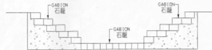
TRAPEZOIDAL CHANNEL WITH GABION BASE AND WALL
