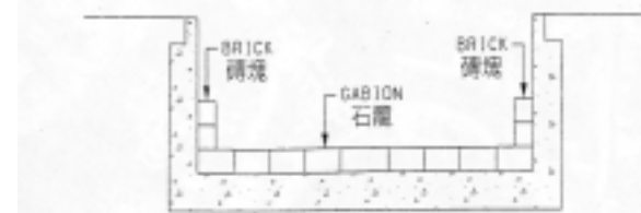
RECTANGULAR CHANNEL WITH GABION BASE AND BRICK WALL
